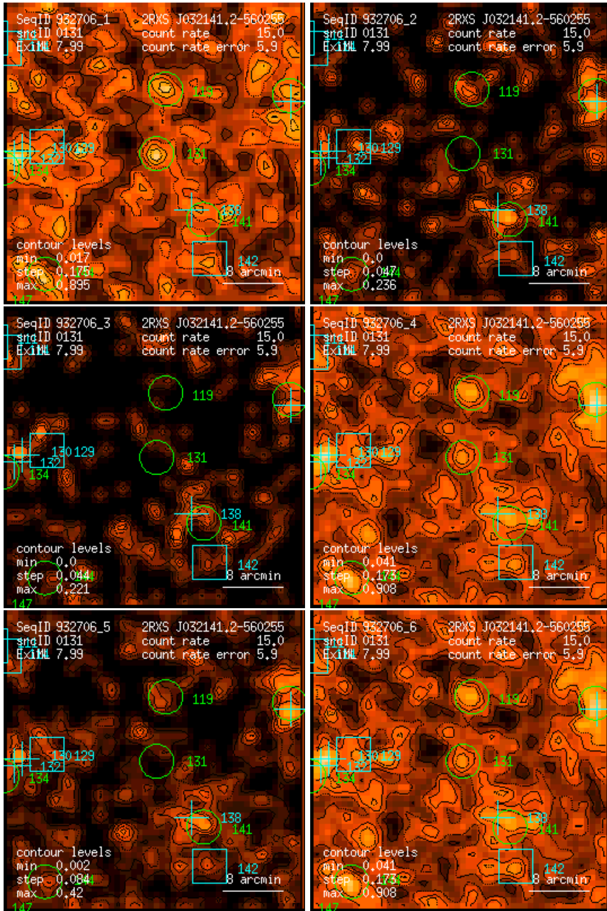
Figure 131: RASS 932706: detection 0131: band rate images, Gaussian filter: (1) PSPC channels 11 – 41, (2) 52 – 90, (3) 91 – 201, (4) 11 – 235, (5) 52 – 201, (6) 11 – 201. Broad band rates in counts/ks. Band rate contour levels in counts/ks/arcmin 2 .
