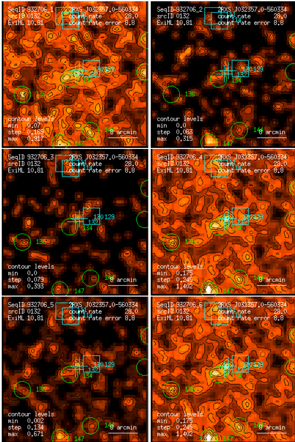
Figure 132: RASS 932706: detection 0132: band rate images, Gaussian filter: (1) PSPC channels 11 – 41, (2) 52 – 90, (3) 91 – 201, (4) 11 – 235, (5) 52 – 201, (6) 11 – 201. Broad band rates in counts/ks. Band rate contour levels in counts/ks/arcmin 2 .
