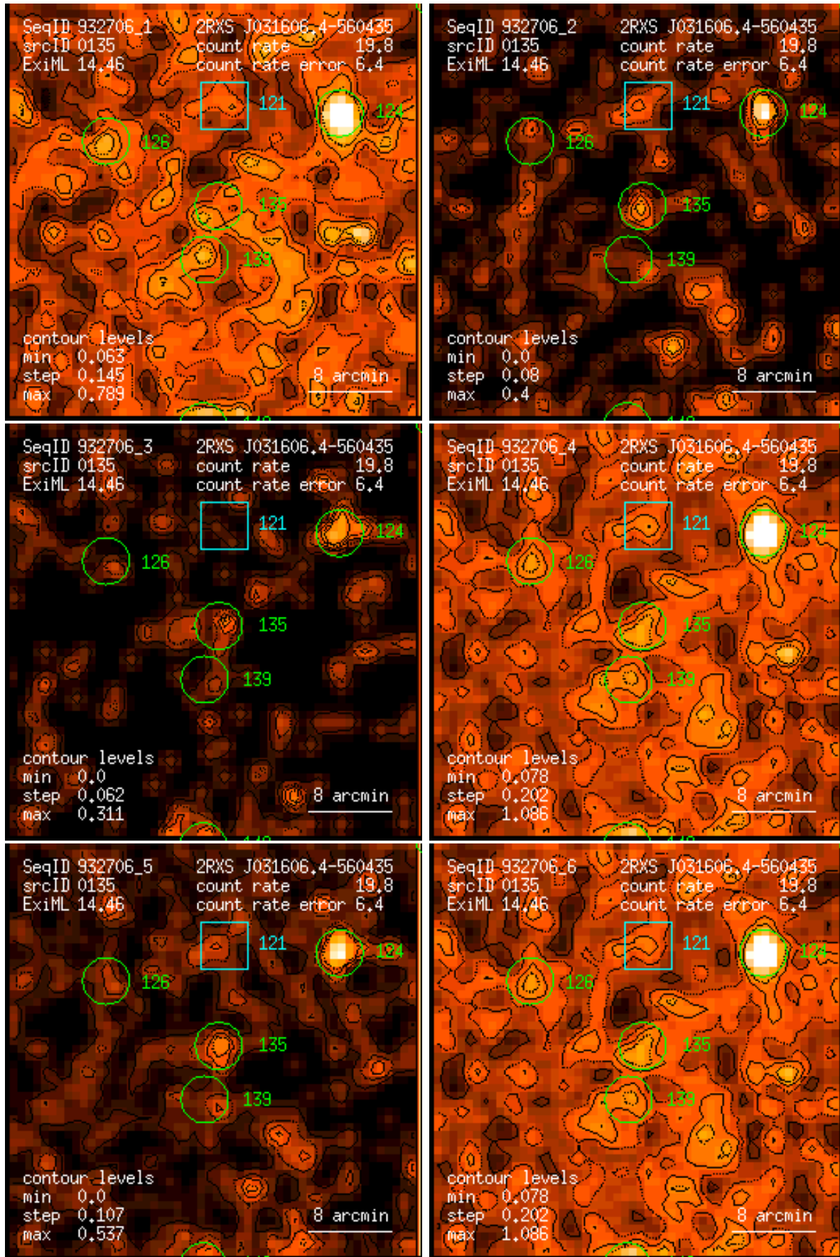
Figure 135: RASS 932706: detection 0135: band rate images, Gaussian filter: (1) PSPC channels 11 – 41, (2) 52 – 90, (3) 91 – 201, (4) 11 – 235, (5) 52 – 201, (6) 11 – 201. Broad band rates in counts/ks. Band rate contour levels in counts/ks/arcmin 2 .
