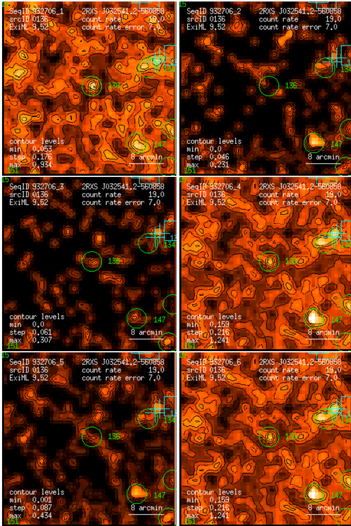
Figure 136: RASS 932706: detection 0136: band rate images, Gaussian filter: (1) PSPC channels 11 – 41, (2) 52 – 90, (3) 91 – 201, (4) 11 – 235, (5) 52 – 201, (6) 11 – 201. Broad band rates in counts/ks. Band rate contour levels in counts/ks/arcmin 2 .
