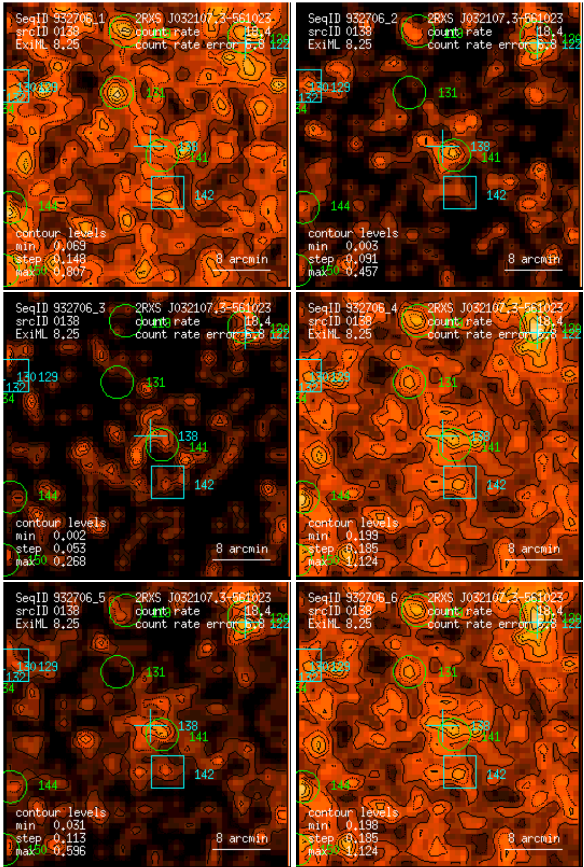
Figure 138: RASS 932706: detection 0138: band rate images, Gaussian filter: (1) PSPC channels 11 – 41, (2) 52 – 90, (3) 91 – 201, (4) 11 – 235, (5) 52 – 201, (6) 11 – 201. Broad band rates in counts/ks. Band rate contour levels in counts/ks/arcmin 2 .
