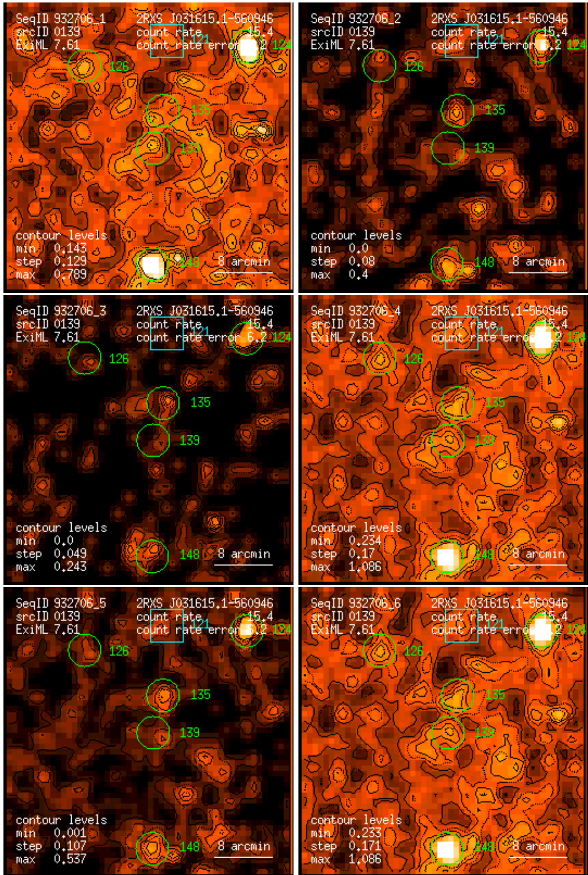
Figure 139: RASS 932706: detection 0139: band rate images, Gaussian filter: (1) PSPC channels 11 – 41, (2) 52 – 90, (3) 91 – 201, (4) 11 – 235, (5) 52 – 201, (6) 11 – 201. Broad band rates in counts/ks. Band rate contour levels in counts/ks/arcmin 2 .
