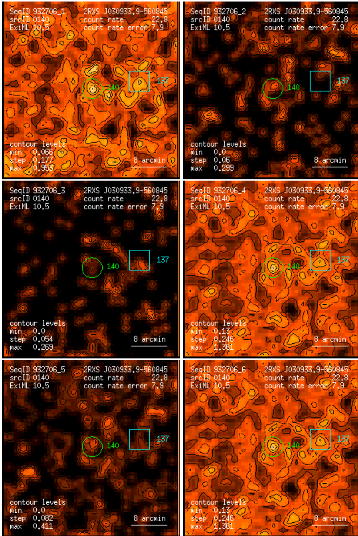
Figure 140: RASS 932706: detection 0140: band rate images, Gaussian filter: (1) PSPC channels 11 – 41, (2) 52 – 90, (3) 91 – 201, (4) 11 – 235, (5) 52 – 201, (6) 11 – 201. Broad band rates in counts/ks. Band rate contour levels in counts/ks/arcmin 2 .
