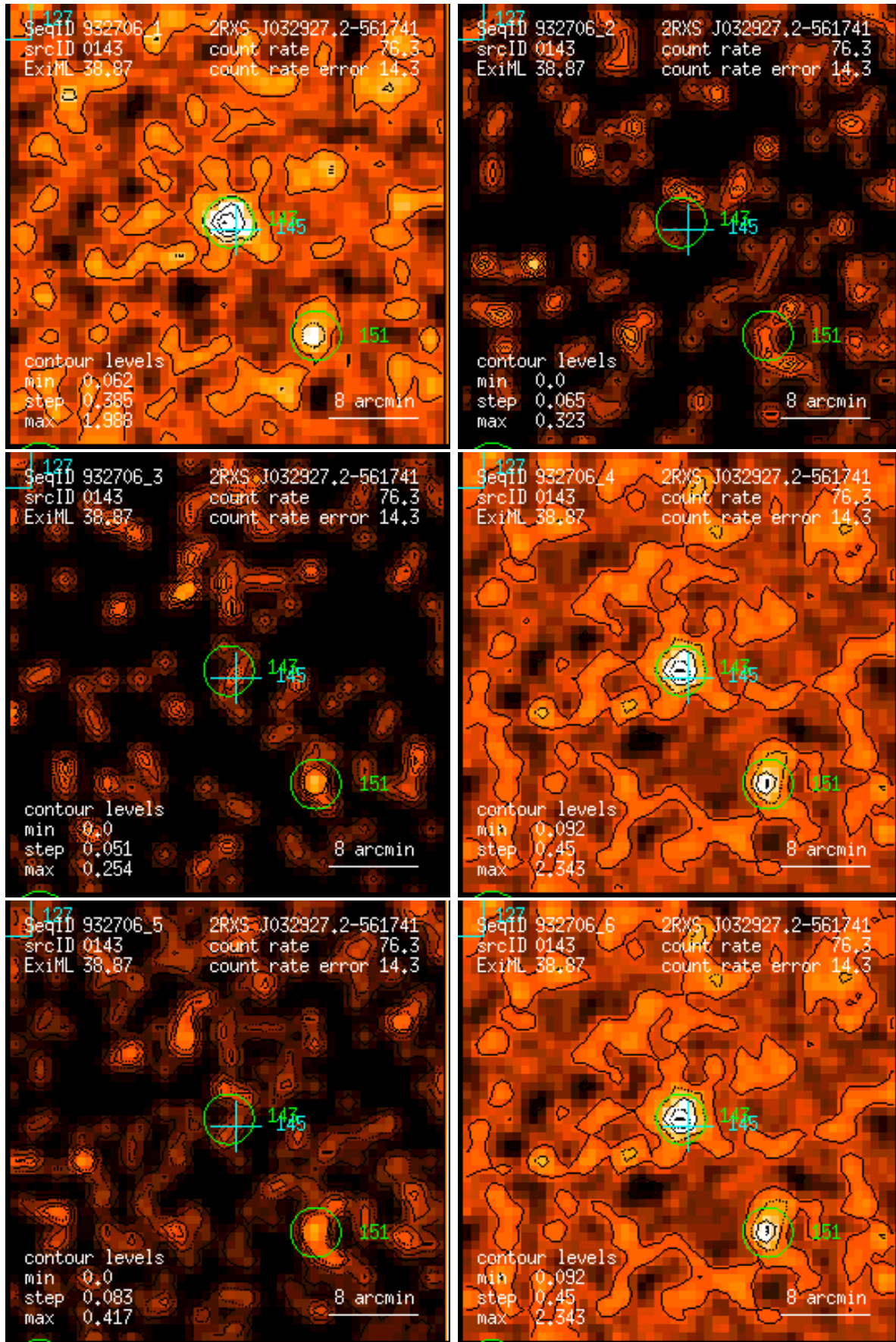
Figure 143: RASS 932706: detection 0143: band rate images, Gaussian filter: (1) PSPC channels 11 – 41, (2) 52 – 90, (3) 91 – 201, (4) 11 – 235, (5) 52 – 201, (6) 11 – 201. Broad band rates in counts/ks. Band rate contour levels in counts/ks/arcmin 2 .
