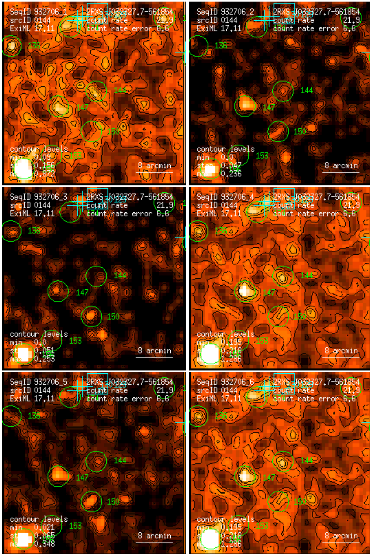
Figure 144: RASS 932706: detection 0144: band rate images, Gaussian filter: (1) PSPC channels 11 – 41, (2) 52 – 90, (3) 91 – 201, (4) 11 – 235, (5) 52 – 201, (6) 11 – 201. Broad band rates in counts/ks. Band rate contour levels in counts/ks/arcmin 2 .
