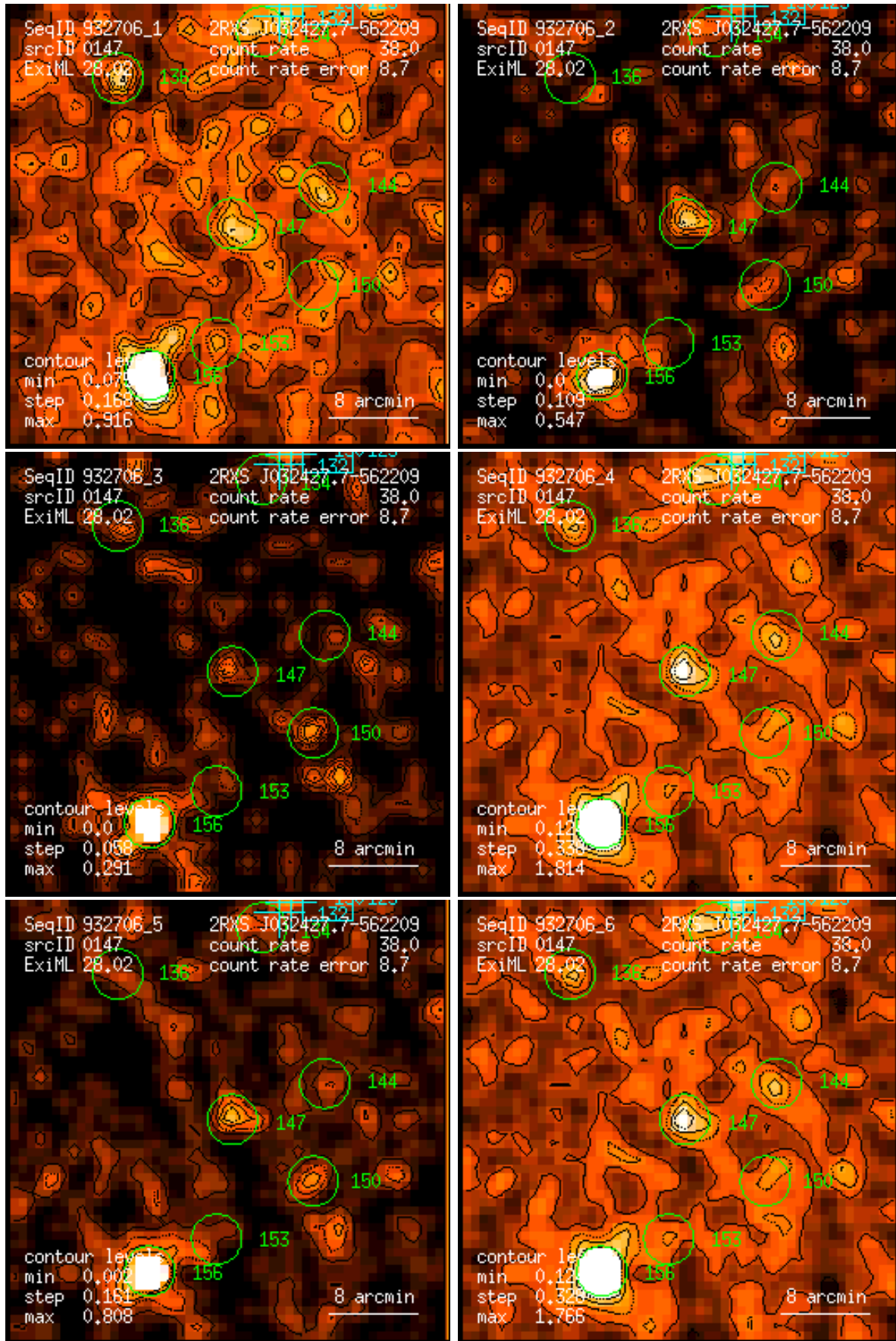
Figure 147: RASS 932706: detection 0147: band rate images, Gaussian filter: (1) PSPC channels 11 – 41, (2) 52 – 90, (3) 91 – 201, (4) 11 – 235, (5) 52 – 201, (6) 11 – 201. Broad band rates in counts/ks. Band rate contour levels in counts/ks/arcmin 2 .
