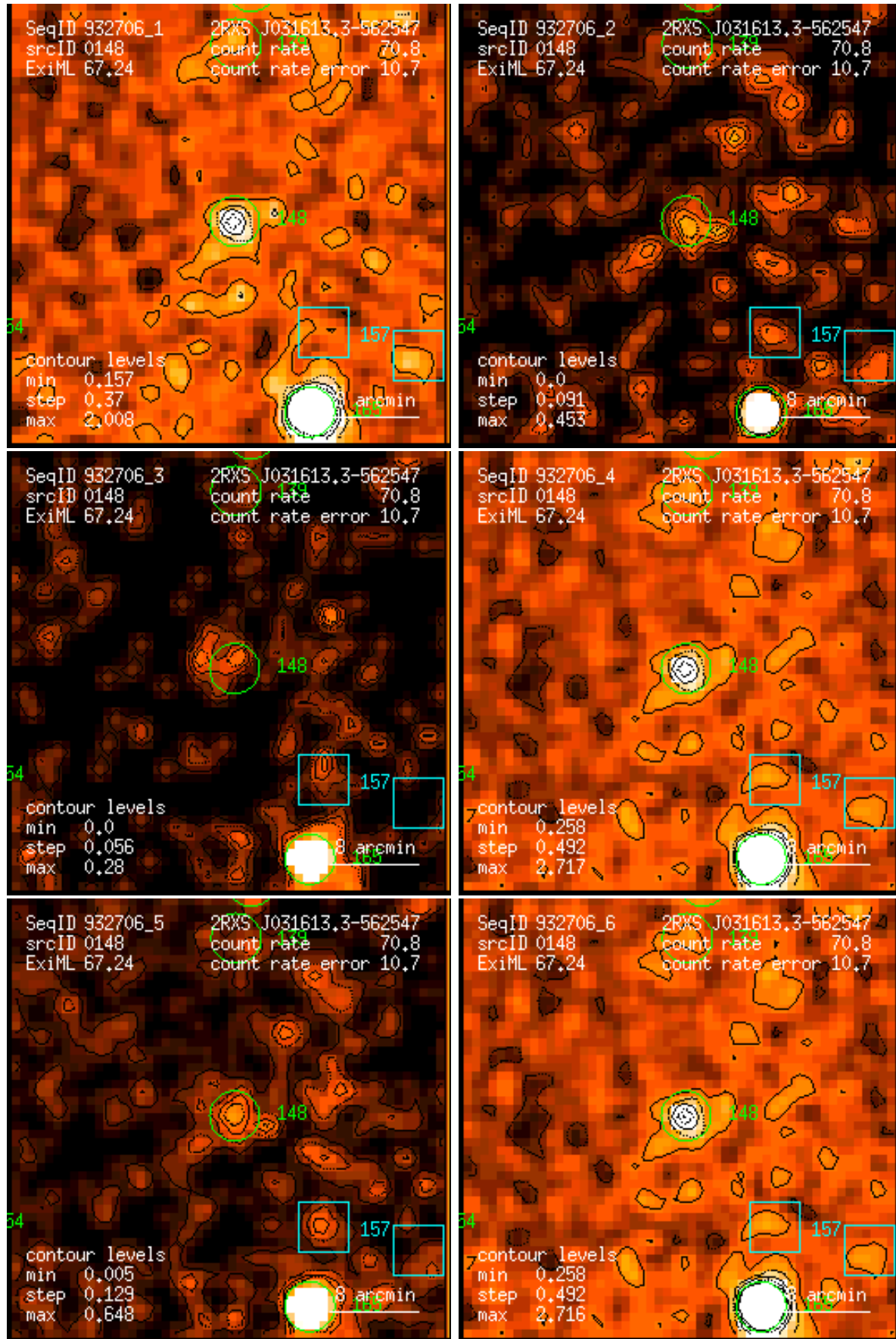
Figure 148: RASS 932706: detection 0148: band rate images, Gaussian filter: (1) PSPC channels 11 – 41, (2) 52 – 90, (3) 91 – 201, (4) 11 – 235, (5) 52 – 201, (6) 11 – 201. Broad band rates in counts/ks. Band rate contour levels in counts/ks/arcmin 2 .
