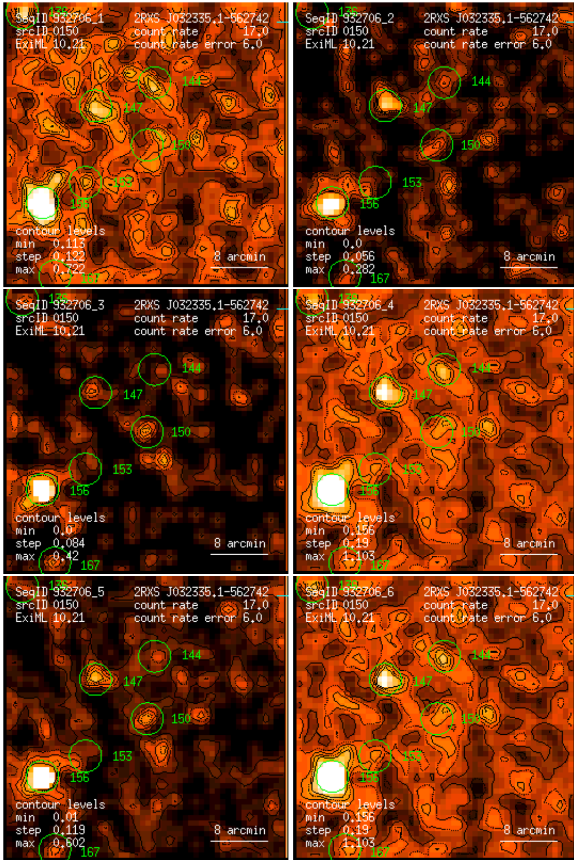
Figure 150: RASS 932706: detection 0150: band rate images, Gaussian filter: (1) PSPC channels 11 – 41, (2) 52 – 90, (3) 91 – 201, (4) 11 – 235, (5) 52 – 201, (6) 11 – 201. Broad band rates in counts/ks. Band rate contour levels in counts/ks/arcmin 2 .
