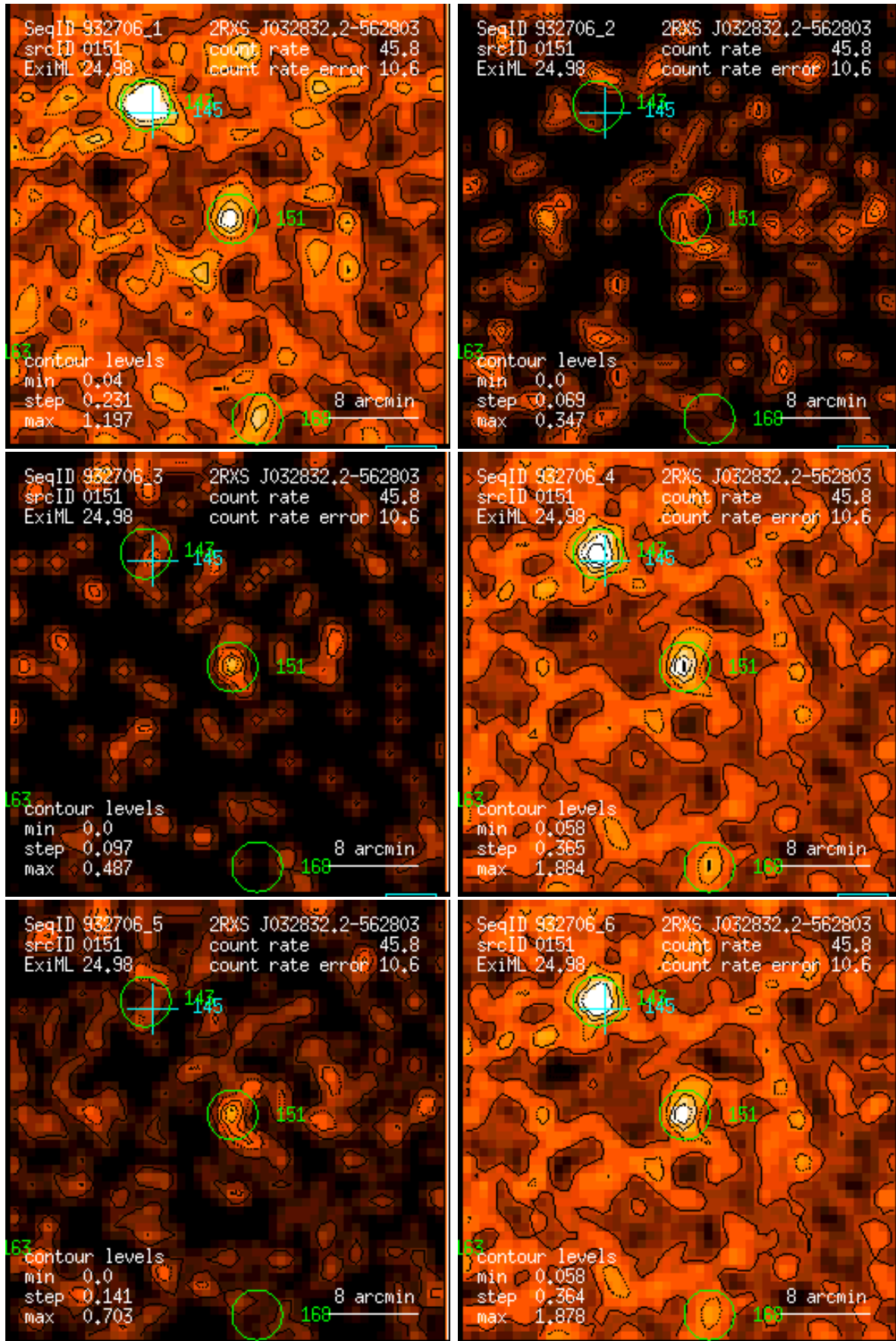
Figure 151: RASS 932706: detection 0151: band rate images, Gaussian filter: (1) PSPC channels 11 – 41, (2) 52 – 90, (3) 91 – 201, (4) 11 – 235, (5) 52 – 201, (6) 11 – 201. Broad band rates in counts/ks. Band rate contour levels in counts/ks/arcmin 2 .
