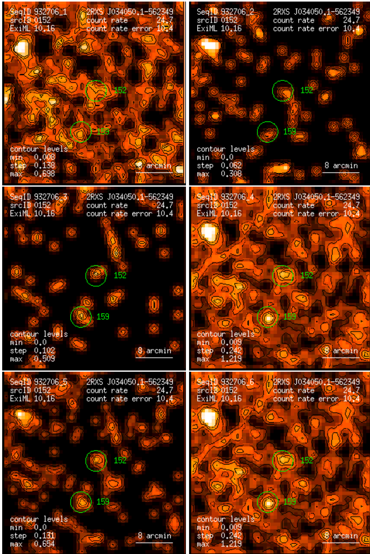
Figure 152: RASS 932706: detection 0152: band rate images, Gaussian filter: (1) PSPC channels 11 – 41, (2) 52 – 90, (3) 91 – 201, (4) 11 – 235, (5) 52 – 201, (6) 11 – 201. Broad band rates in counts/ks. Band rate contour levels in counts/ks/arcmin 2 .
