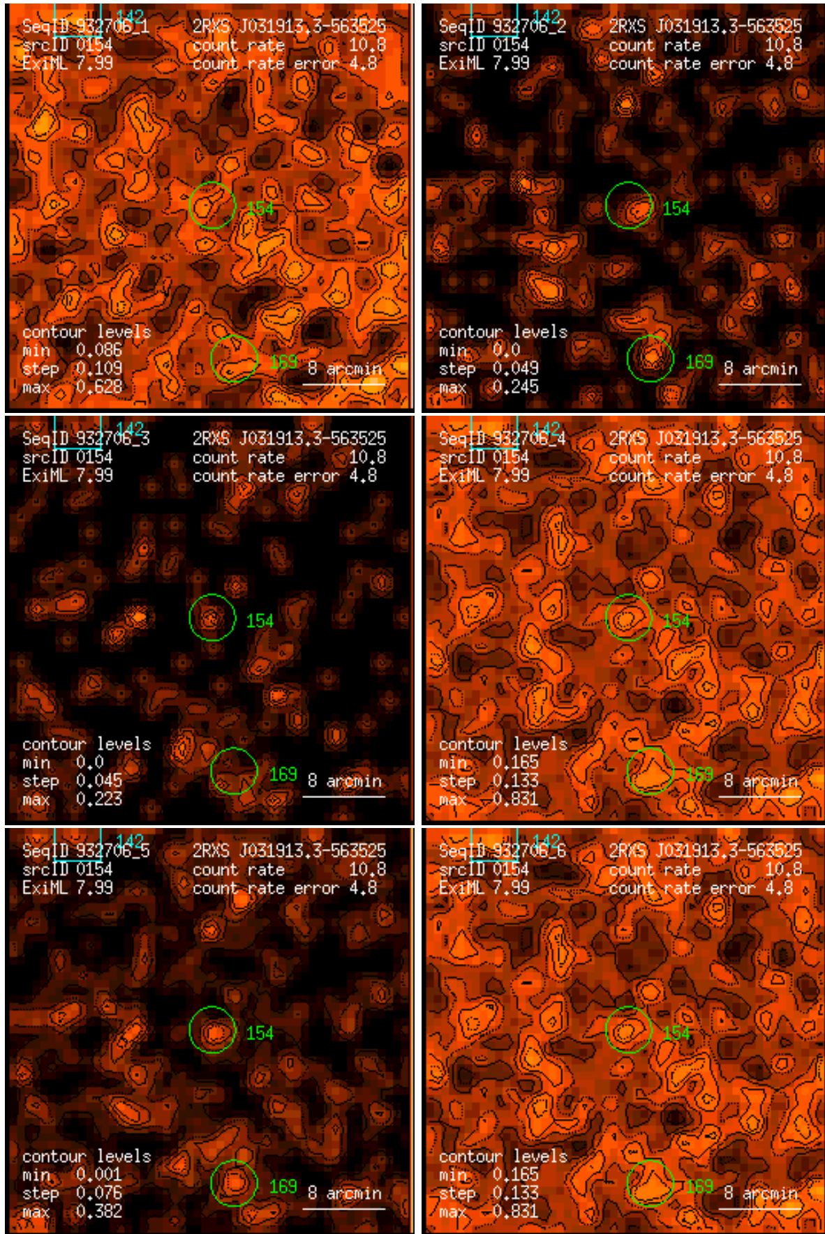
Figure 154: RASS 932706: detection 0154: band rate images, Gaussian filter: (1) PSPC channels 11 – 41, (2) 52 – 90, (3) 91 – 201, (4) 11 – 235, (5) 52 – 201, (6) 11 – 201. Broad band rates in counts/ks. Band rate contour levels in counts/ks/arcmin 2 .
