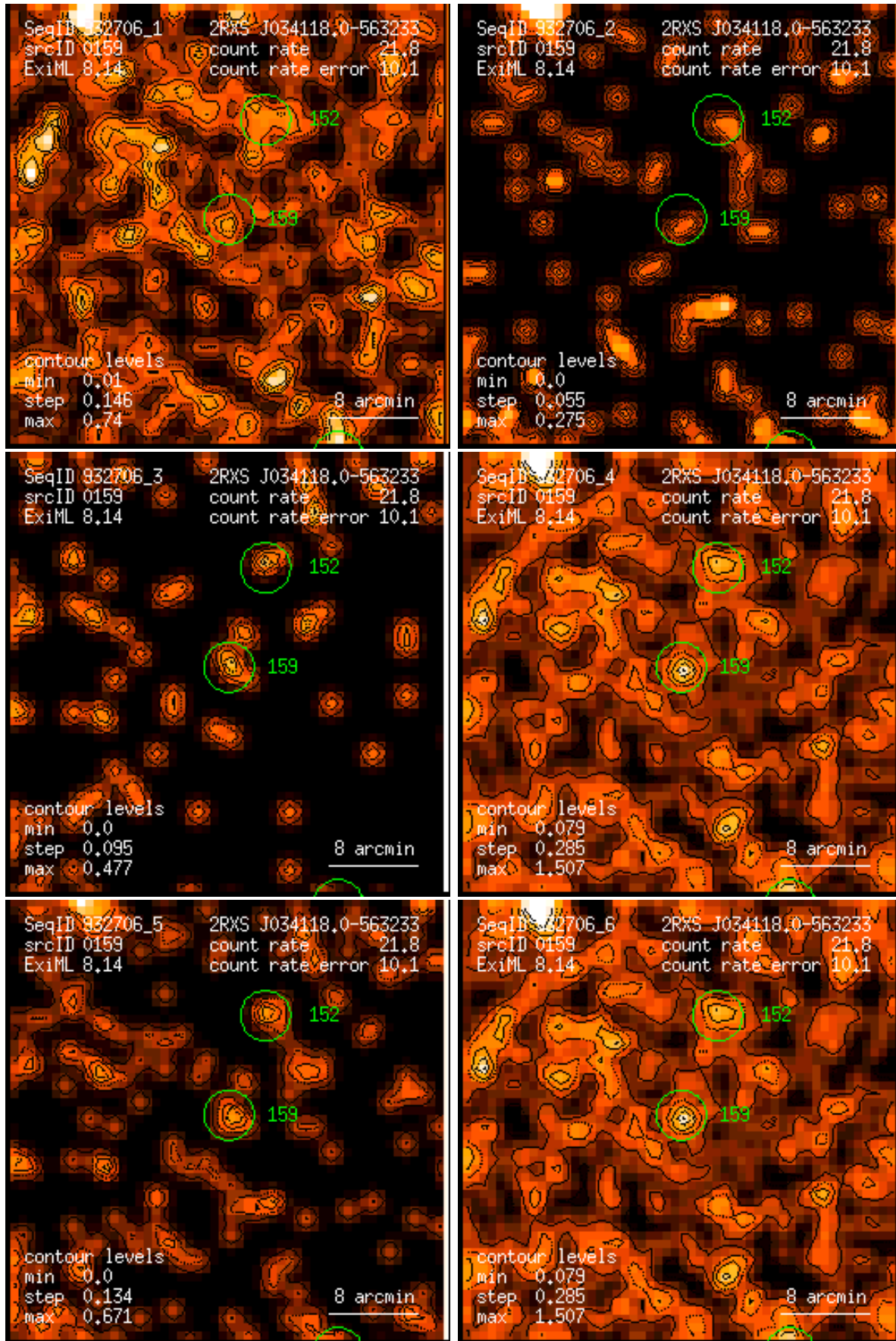
Figure 159: RASS 932706: detection 0159: band rate images, Gaussian filter: (1) PSPC channels 11 – 41, (2) 52 – 90, (3) 91 – 201, (4) 11 – 235, (5) 52 – 201, (6) 11 – 201. Broad band rates in counts/ks. Band rate contour levels in counts/ks/arcmin 2 .
