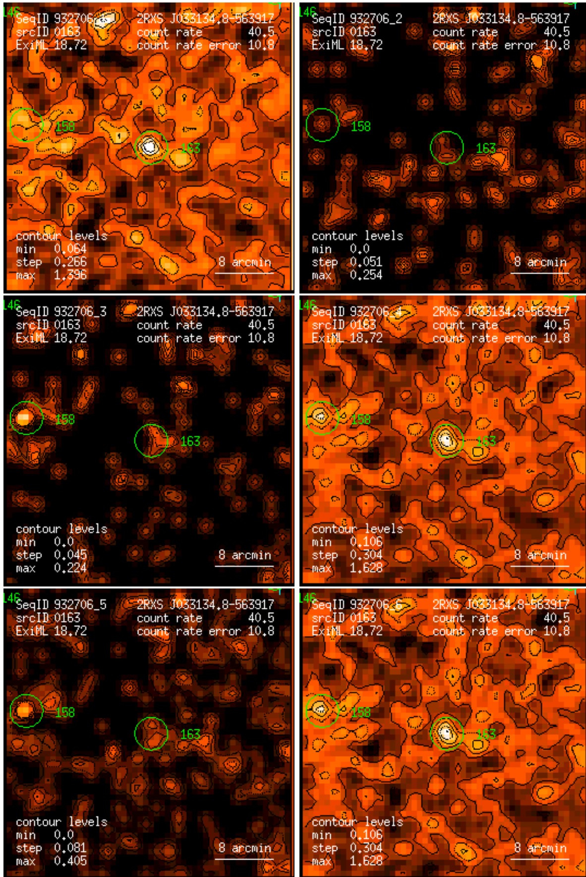
Figure 163: RASS 932706: detection 0163: band rate images, Gaussian filter: (1) PSPC channels 11 – 41, (2) 52 – 90, (3) 91 – 201, (4) 11 – 235, (5) 52 – 201, (6) 11 – 201. Broad band rates in counts/ks. Band rate contour levels in counts/ks/arcmin 2 .
