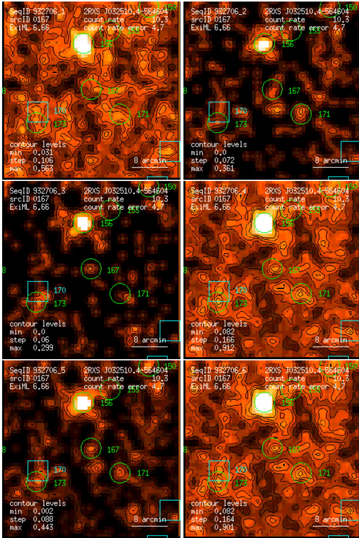
Figure 167: RASS 932706: detection 0167: band rate images, Gaussian filter: (1) PSPC channels 11 – 41, (2) 52 – 90, (3) 91 – 201, (4) 11 – 235, (5) 52 – 201, (6) 11 – 201. Broad band rates in counts/ks. Band rate contour levels in counts/ks/arcmin 2 .
