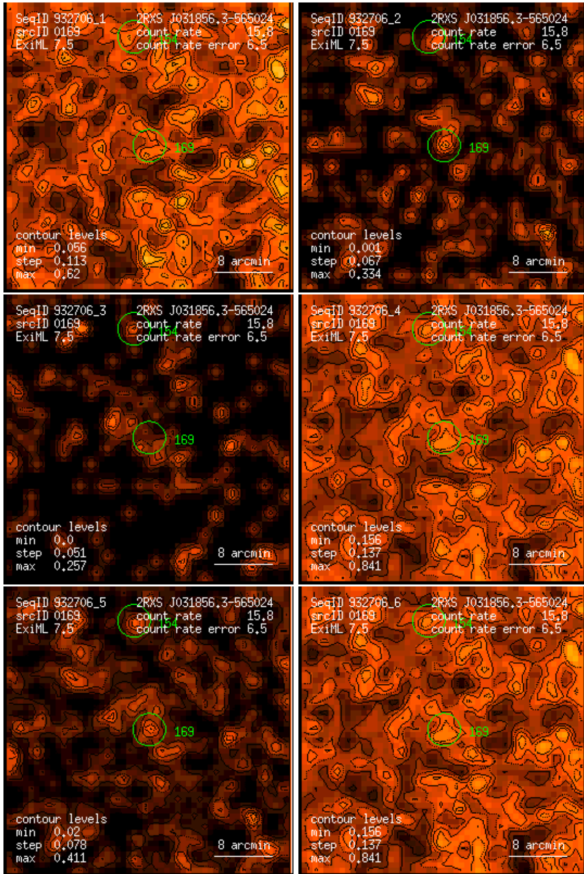
Figure 169: RASS 932706: detection 0169: band rate images, Gaussian filter: (1) PSPC channels 11 – 41, (2) 52 – 90, (3) 91 – 201, (4) 11 – 235, (5) 52 – 201, (6) 11 – 201. Broad band rates in counts/ks. Band rate contour levels in counts/ks/arcmin 2 .
