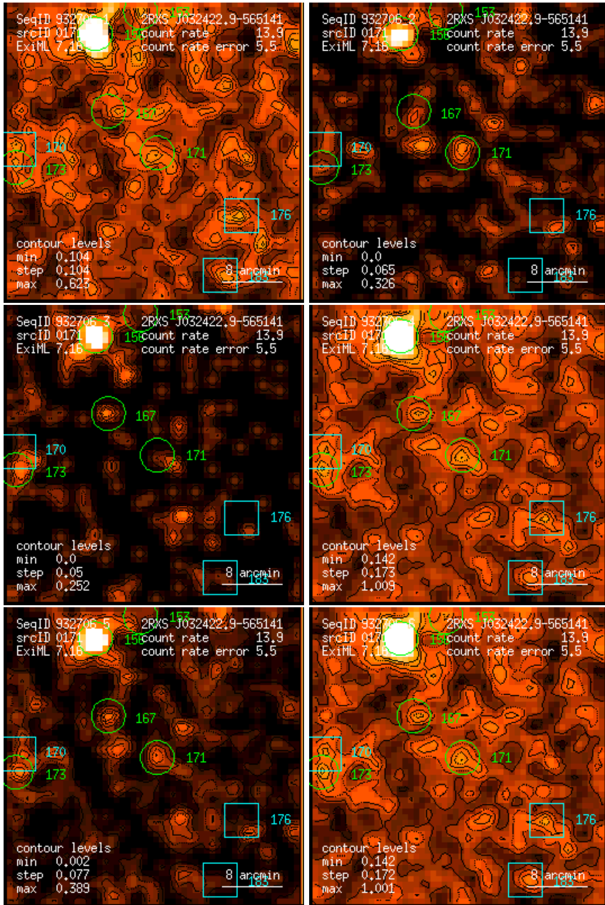
Figure 171: RASS 932706: detection 0171: band rate images, Gaussian filter: (1) PSPC channels 11 – 41, (2) 52 – 90, (3) 91 – 201, (4) 11 – 235, (5) 52 – 201, (6) 11 – 201. Broad band rates in counts/ks. Band rate contour levels in counts/ks/arcmin 2 .
