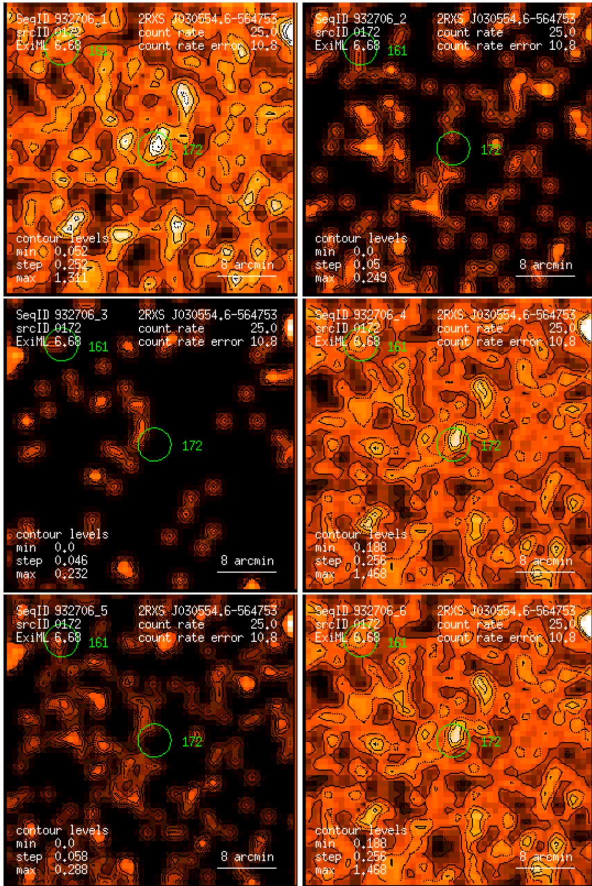
Figure 172: RASS 932706: detection 0172: band rate images, Gaussian filter: (1) PSPC channels 11 – 41, (2) 52 – 90, (3) 91 – 201, (4) 11 – 235, (5) 52 – 201, (6) 11 – 201. Broad band rates in counts/ks. Band rate contour levels in counts/ks/arcmin 2 .
