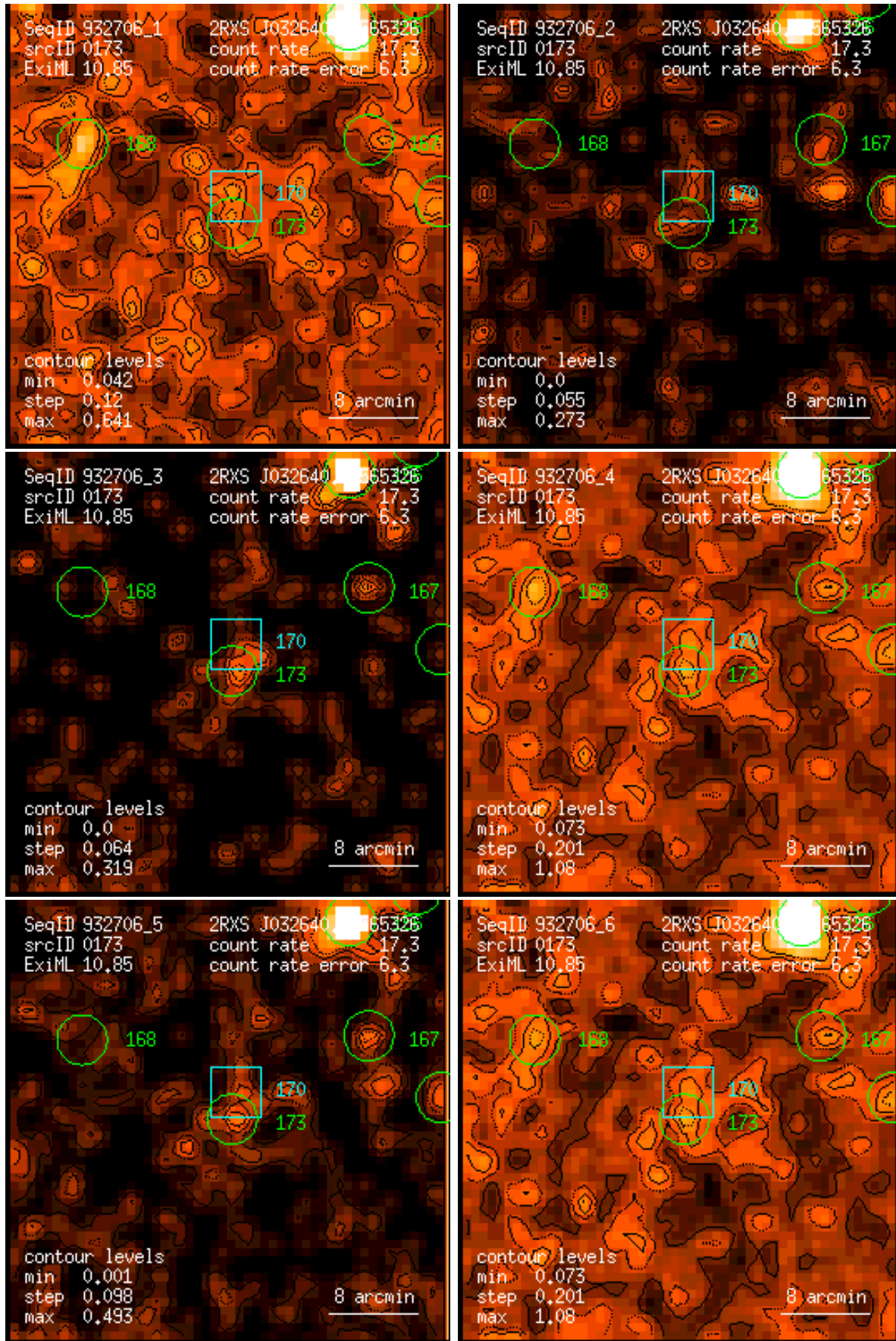
Figure 173: RASS 932706: detection 0173: band rate images, Gaussian filter: (1) PSPC channels 11 – 41, (2) 52 – 90, (3) 91 – 201, (4) 11 – 235, (5) 52 – 201, (6) 11 – 201. Broad band rates in counts/ks. Band rate contour levels in counts/ks/arcmin 2 .
