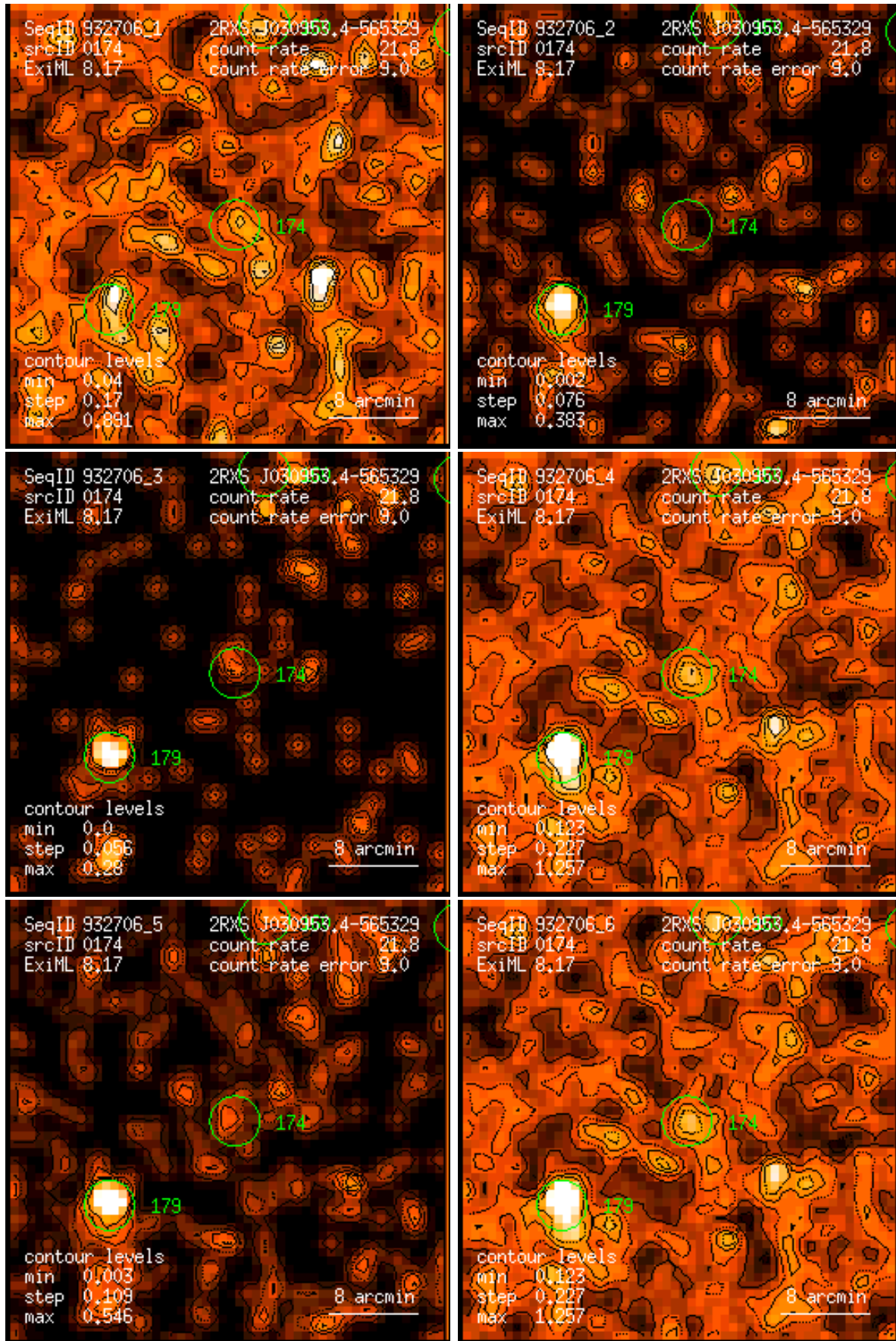
Figure 174: RASS 932706: detection 0174: band rate images, Gaussian filter: (1) PSPC channels 11 – 41, (2) 52 – 90, (3) 91 – 201, (4) 11 – 235, (5) 52 – 201, (6) 11 – 201. Broad band rates in counts/ks. Band rate contour levels in counts/ks/arcmin 2 .
