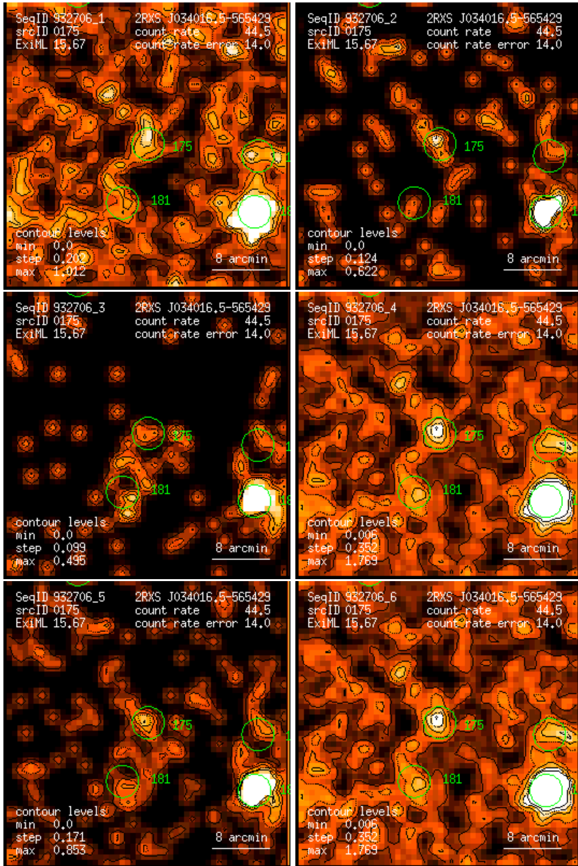
Figure 175: RASS 932706: detection 0175: band rate images, Gaussian filter: (1) PSPC channels 11 – 41, (2) 52 – 90, (3) 91 – 201, (4) 11 – 235, (5) 52 – 201, (6) 11 – 201. Broad band rates in counts/ks. Band rate contour levels in counts/ks/arcmin 2 .
