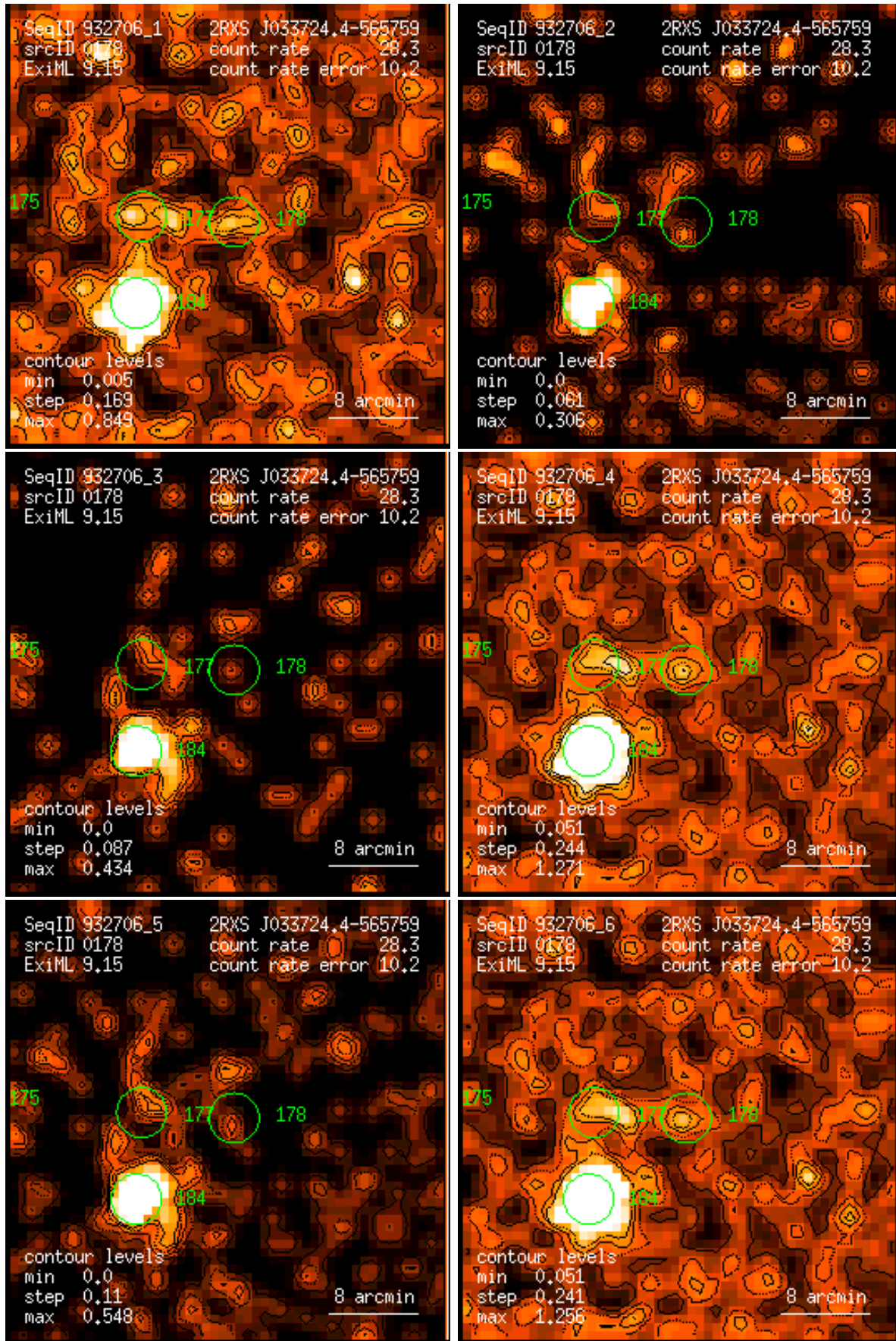
Figure 178: RASS 932706: detection 0178: band rate images, Gaussian filter: (1) PSPC channels 11 – 41, (2) 52 – 90, (3) 91 – 201, (4) 11 – 235, (5) 52 – 201, (6) 11 – 201. Broad band rates in counts/ks. Band rate contour levels in counts/ks/arcmin 2 .
