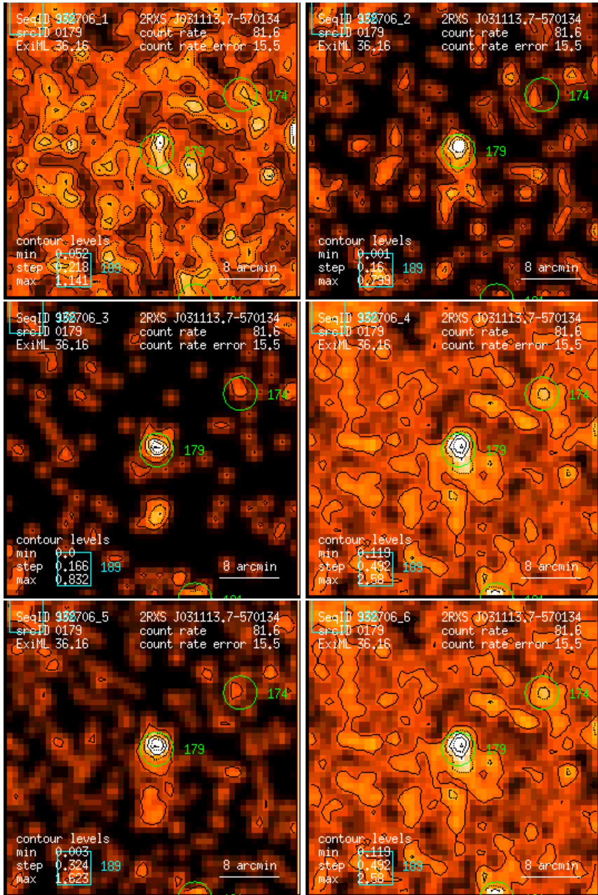
Figure 179: RASS 932706: detection 0179: band rate images, Gaussian filter: (1) PSPC channels 11 – 41, (2) 52 – 90, (3) 91 – 201, (4) 11 – 235, (5) 52 – 201, (6) 11 – 201. Broad band rates in counts/ks. Band rate contour levels in counts/ks/arcmin 2 .
