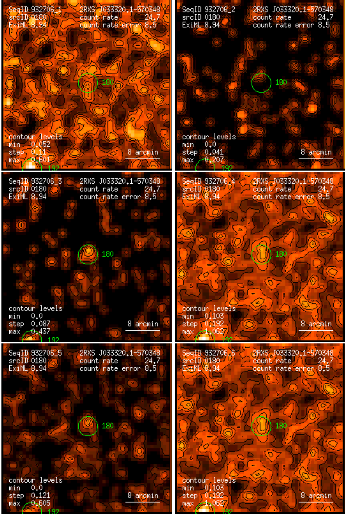
Figure 180: RASS 932706: detection 0180: band rate images, Gaussian filter: (1) PSPC channels 11 – 41, (2) 52 – 90, (3) 91 – 201, (4) 11 – 235, (5) 52 – 201, (6) 11 – 201. Broad band rates in counts/ks. Band rate contour levels in counts/ks/arcmin 2 .
