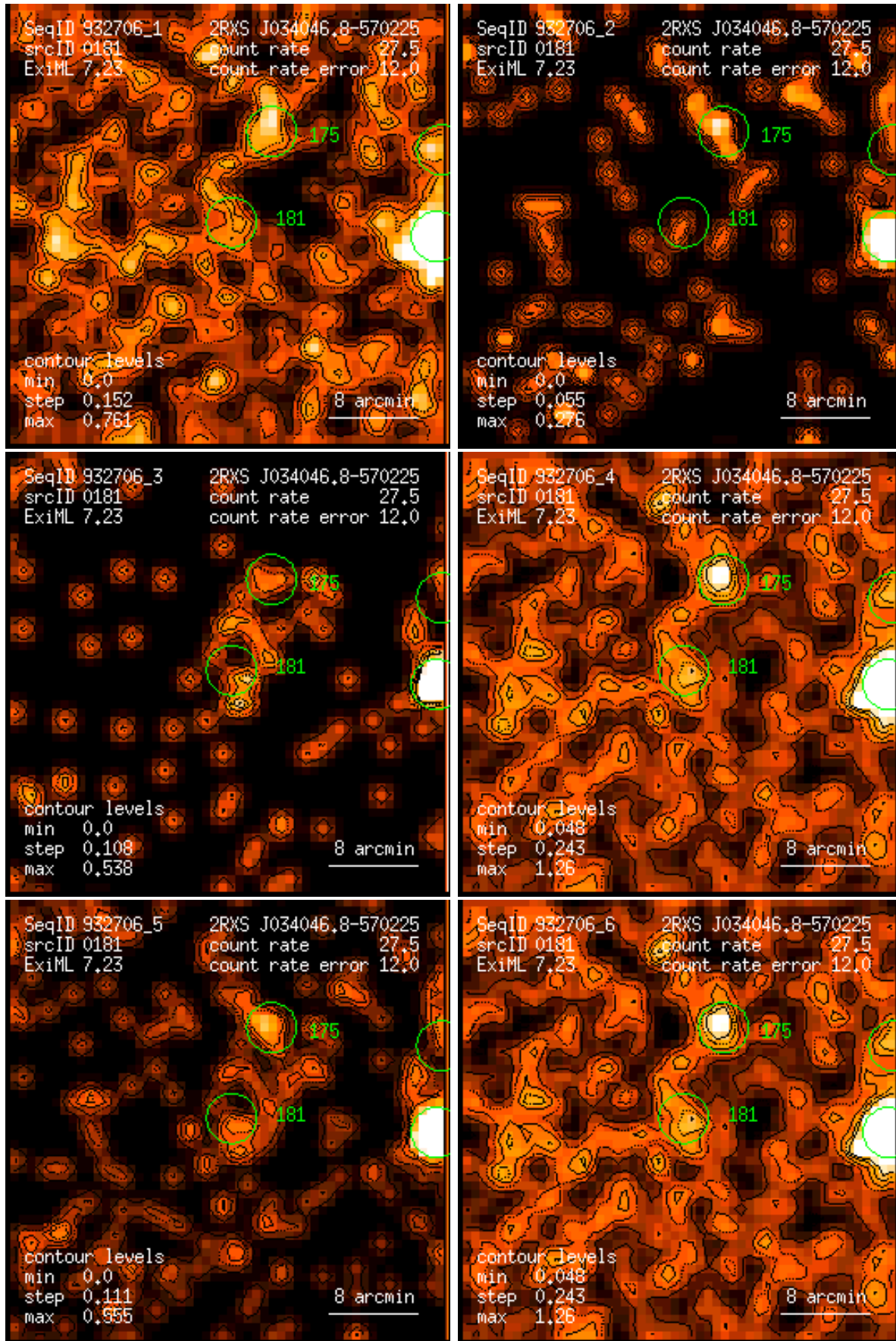
Figure 181: RASS 932706: detection 0181: band rate images, Gaussian filter: (1) PSPC channels 11 – 41, (2) 52 – 90, (3) 91 – 201, (4) 11 – 235, (5) 52 – 201, (6) 11 – 201. Broad band rates in counts/ks. Band rate contour levels in counts/ks/arcmin 2 .
