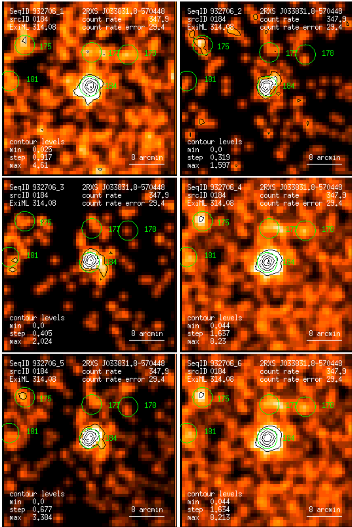
Figure 184: RASS 932706: detection 0184: band rate images, Gaussian filter: (1) PSPC channels 11 – 41, (2) 52 – 90, (3) 91 – 201, (4) 11 – 235, (5) 52 – 201, (6) 11 – 201. Broad band rates in counts/ks. Band rate contour levels in counts/ks/arcmin 2 .
