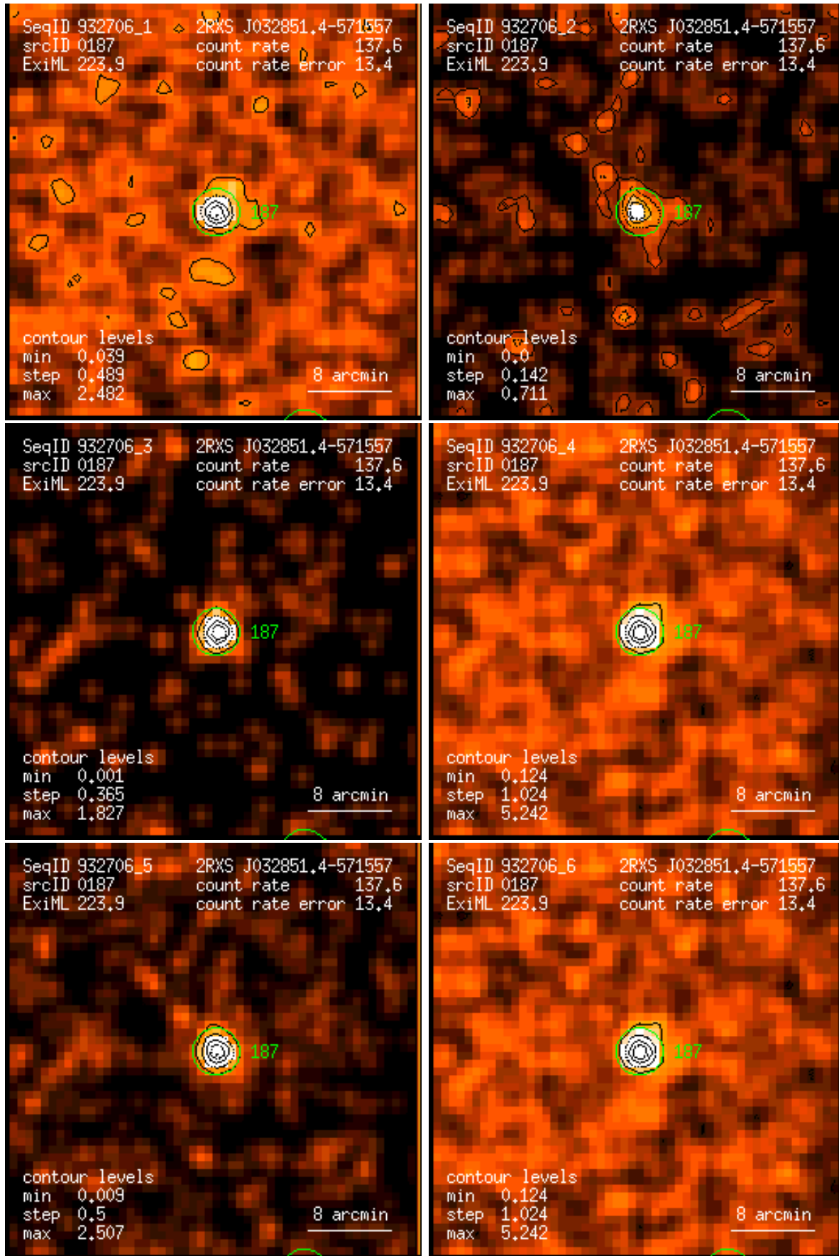
Figure 187: RASS 932706: detection 0187: band rate images, Gaussian filter: (1) PSPC channels 11 – 41, (2) 52 – 90, (3) 91 – 201, (4) 11 – 235, (5) 52 – 201, (6) 11 – 201. Broad band rates in counts/ks. Band rate contour levels in counts/ks/arcmin 2 .
