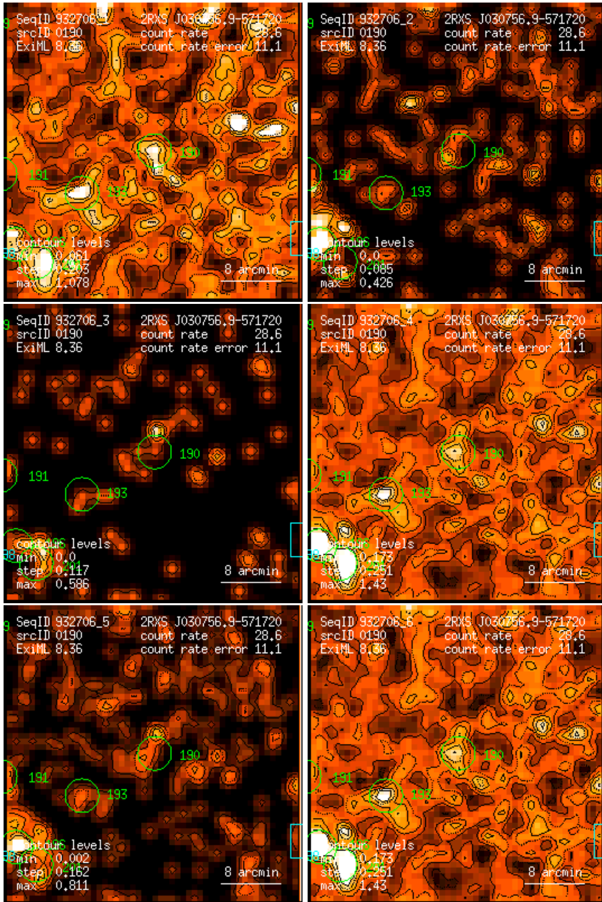
Figure 190: RASS 932706: detection 0190: band rate images, Gaussian filter: (1) PSPC channels 11 – 41, (2) 52 – 90, (3) 91 – 201, (4) 11 – 235, (5) 52 – 201, (6) 11 – 201. Broad band rates in counts/ks. Band rate contour levels in counts/ks/arcmin 2 .
