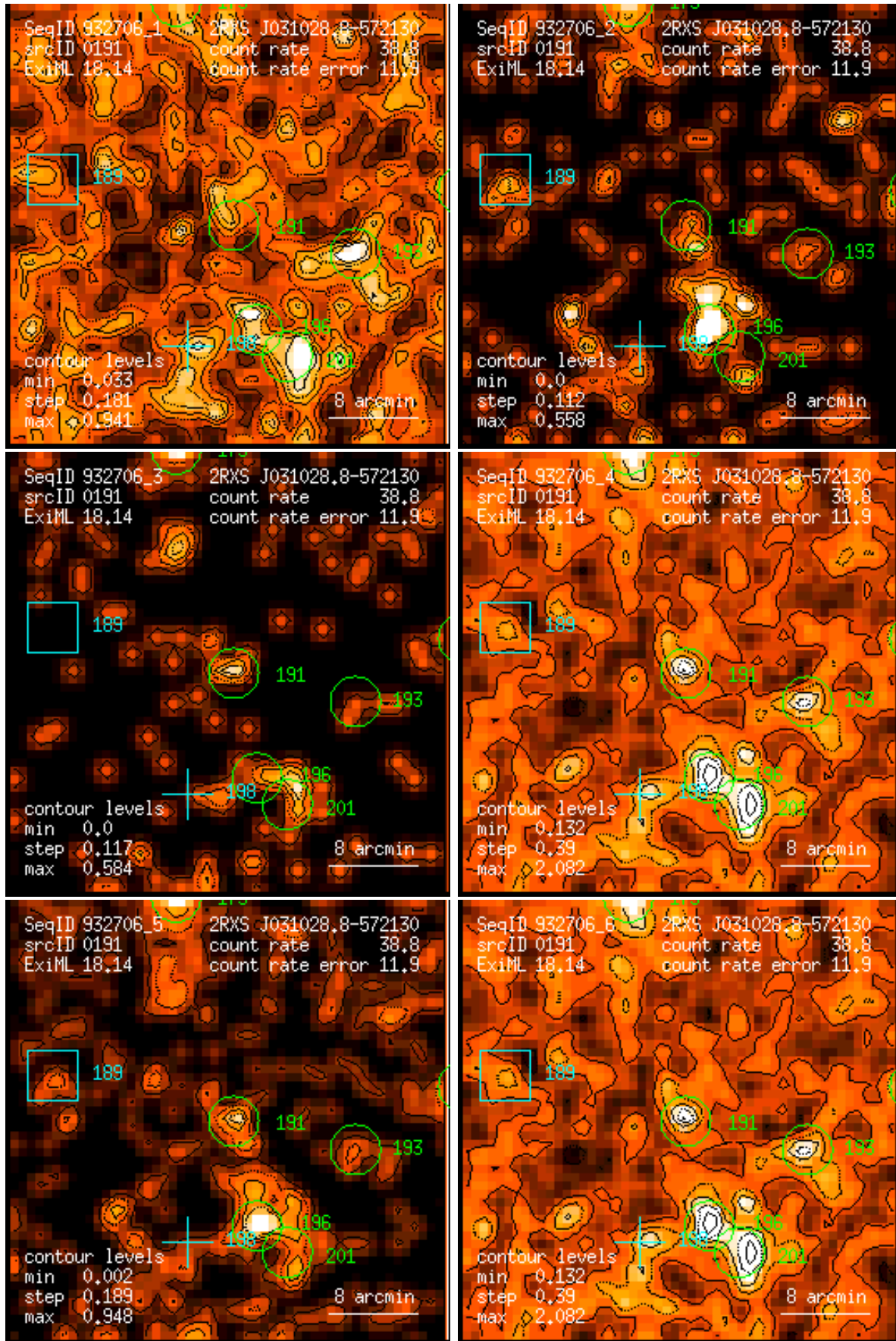
Figure 191: RASS 932706: detection 0191: band rate images, Gaussian filter: (1) PSPC channels 11 – 41, (2) 52 – 90, (3) 91 – 201, (4) 11 – 235, (5) 52 – 201, (6) 11 – 201. Broad band rates in counts/ks. Band rate contour levels in counts/ks/arcmin 2 .
