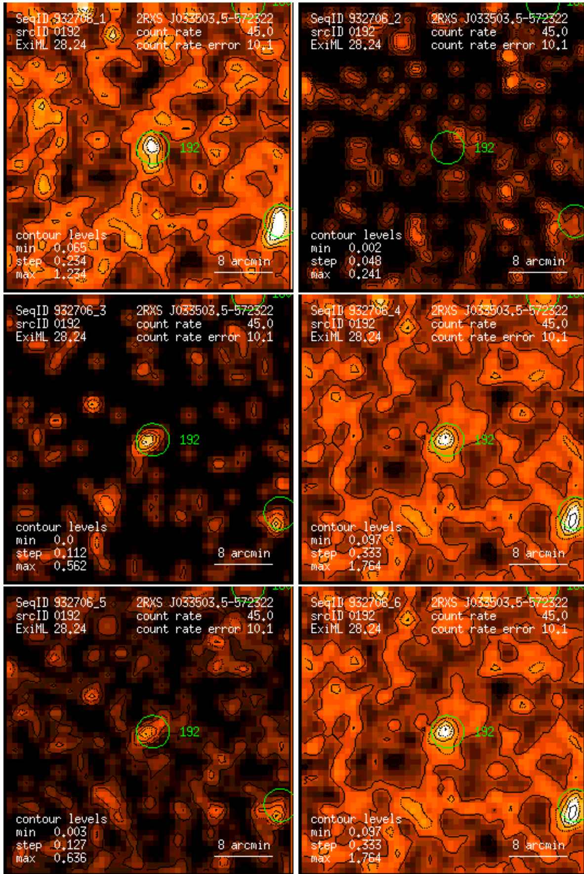
Figure 192: RASS 932706: detection 0192: band rate images, Gaussian filter: (1) PSPC channels 11 – 41, (2) 52 – 90, (3) 91 – 201, (4) 11 – 235, (5) 52 – 201, (6) 11 – 201. Broad band rates in counts/ks. Band rate contour levels in counts/ks/arcmin 2 .
