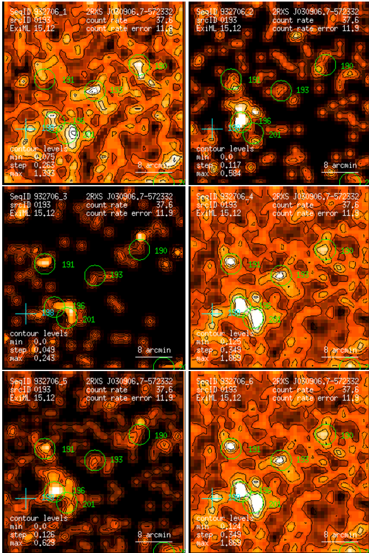
Figure 193: RASS 932706: detection 0193: band rate images, Gaussian filter: (1) PSPC channels 11 – 41, (2) 52 – 90, (3) 91 – 201, (4) 11 – 235, (5) 52 – 201, (6) 11 – 201. Broad band rates in counts/ks. Band rate contour levels in counts/ks/arcmin 2 .
