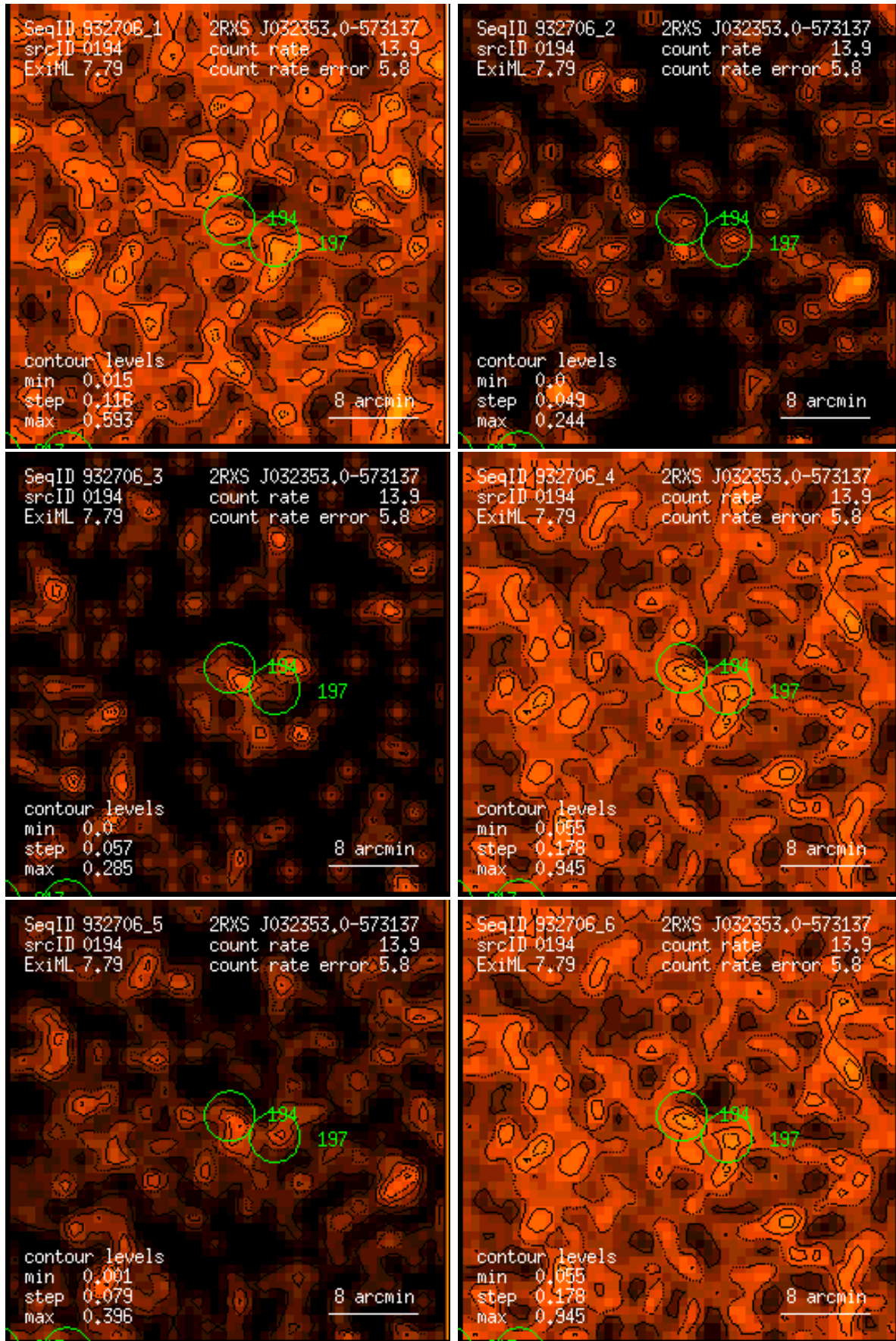
Figure 194: RASS 932706: detection 0194: band rate images, Gaussian filter: (1) PSPC channels 11 – 41, (2) 52 – 90, (3) 91 – 201, (4) 11 – 235, (5) 52 – 201, (6) 11 – 201. Broad band rates in counts/ks. Band rate contour levels in counts/ks/arcmin 2 .
