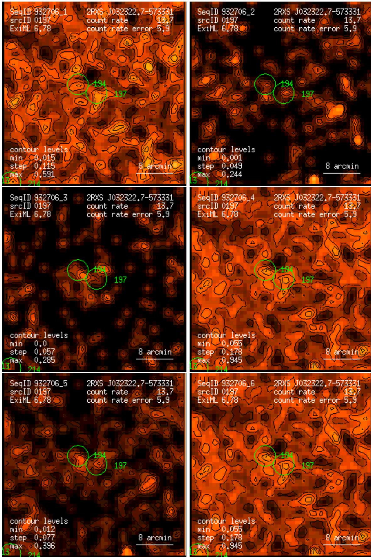
Figure 197: RASS 932706: detection 0197: band rate images, Gaussian filter: (1) PSPC channels 11 – 41, (2) 52 – 90, (3) 91 – 201, (4) 11 – 235, (5) 52 – 201, (6) 11 – 201. Broad band rates in counts/ks. Band rate contour levels in counts/ks/arcmin 2 .
