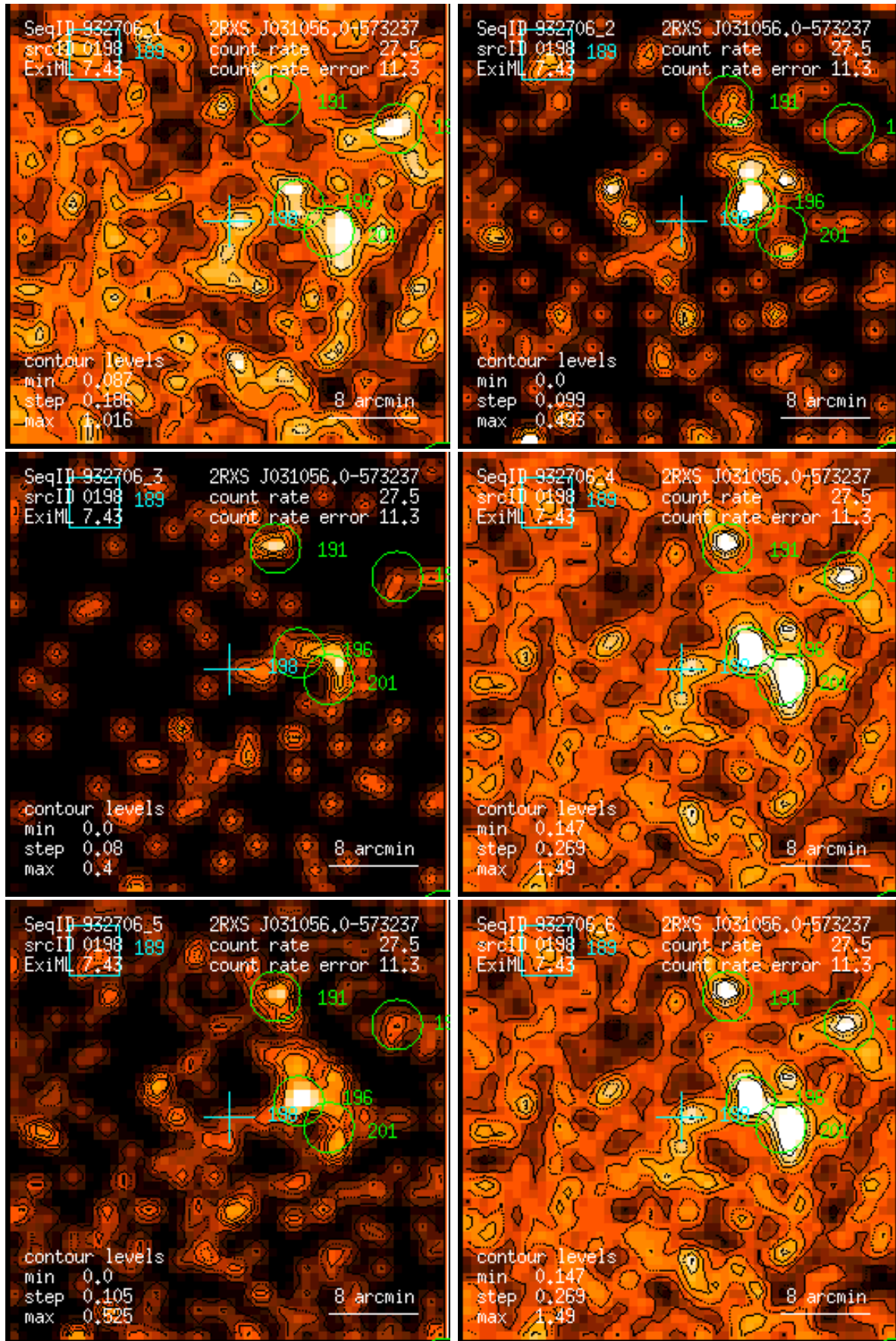
Figure 198: RASS 932706: detection 0198: band rate images, Gaussian filter: (1) PSPC channels 11 – 41, (2) 52 – 90, (3) 91 – 201, (4) 11 – 235, (5) 52 – 201, (6) 11 – 201. Broad band rates in counts/ks. Band rate contour levels in counts/ks/arcmin 2 .
