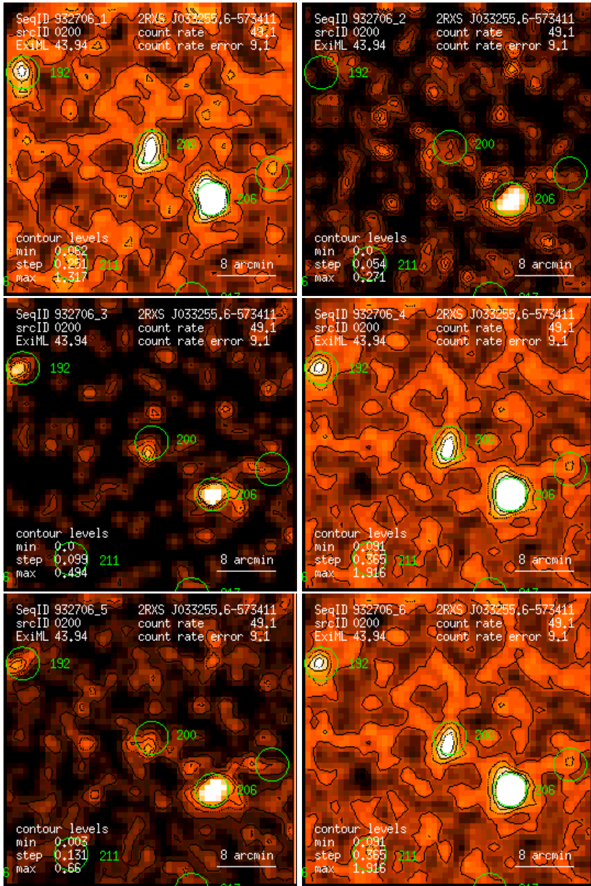
Figure 200: RASS 932706: detection 0200: band rate images, Gaussian filter: (1) PSPC channels 11 – 41, (2) 52 – 90, (3) 91 – 201, (4) 11 – 235, (5) 52 – 201, (6) 11 – 201. Broad band rates in counts/ks. Band rate contour levels in counts/ks/arcmin 2 .
