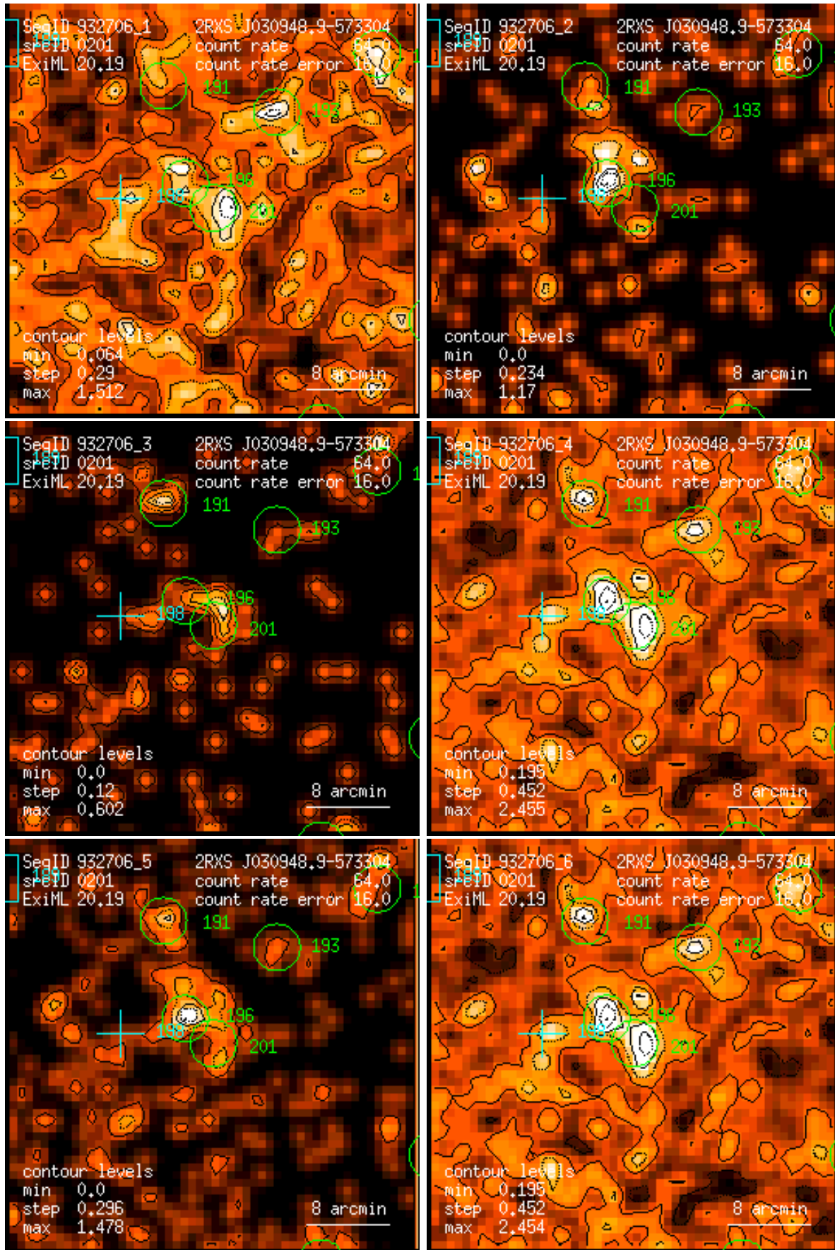
Figure 201: RASS 932706: detection 0201: band rate images, Gaussian filter: (1) PSPC channels 11 – 41, (2) 52 – 90, (3) 91 – 201, (4) 11 – 235, (5) 52 – 201, (6) 11 – 201. Broad band rates in counts/ks. Band rate contour levels in counts/ks/arcmin 2 .
