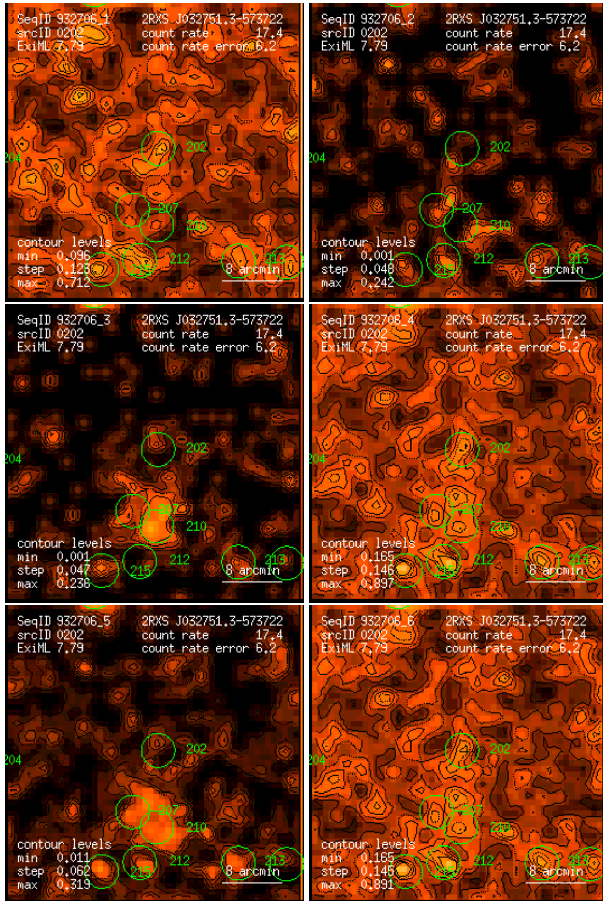
Figure 202: RASS 932706: detection 0202: band rate images, Gaussian filter: (1) PSPC channels 11 – 41, (2) 52 – 90, (3) 91 – 201, (4) 11 – 235, (5) 52 – 201, (6) 11 – 201. Broad band rates in counts/ks. Band rate contour levels in counts/ks/arcmin 2 .
