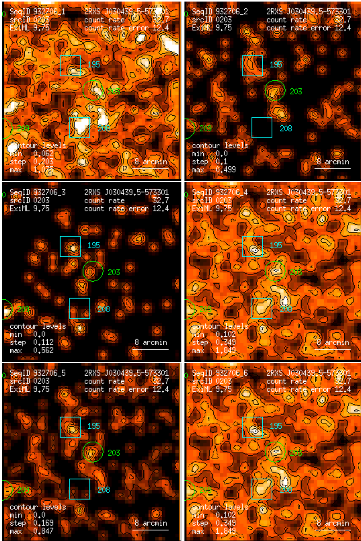
Figure 203: RASS 932706: detection 0203: band rate images, Gaussian filter: (1) PSPC channels 11 – 41, (2) 52 – 90, (3) 91 – 201, (4) 11 – 235, (5) 52 – 201, (6) 11 – 201. Broad band rates in counts/ks. Band rate contour levels in counts/ks/arcmin 2 .
