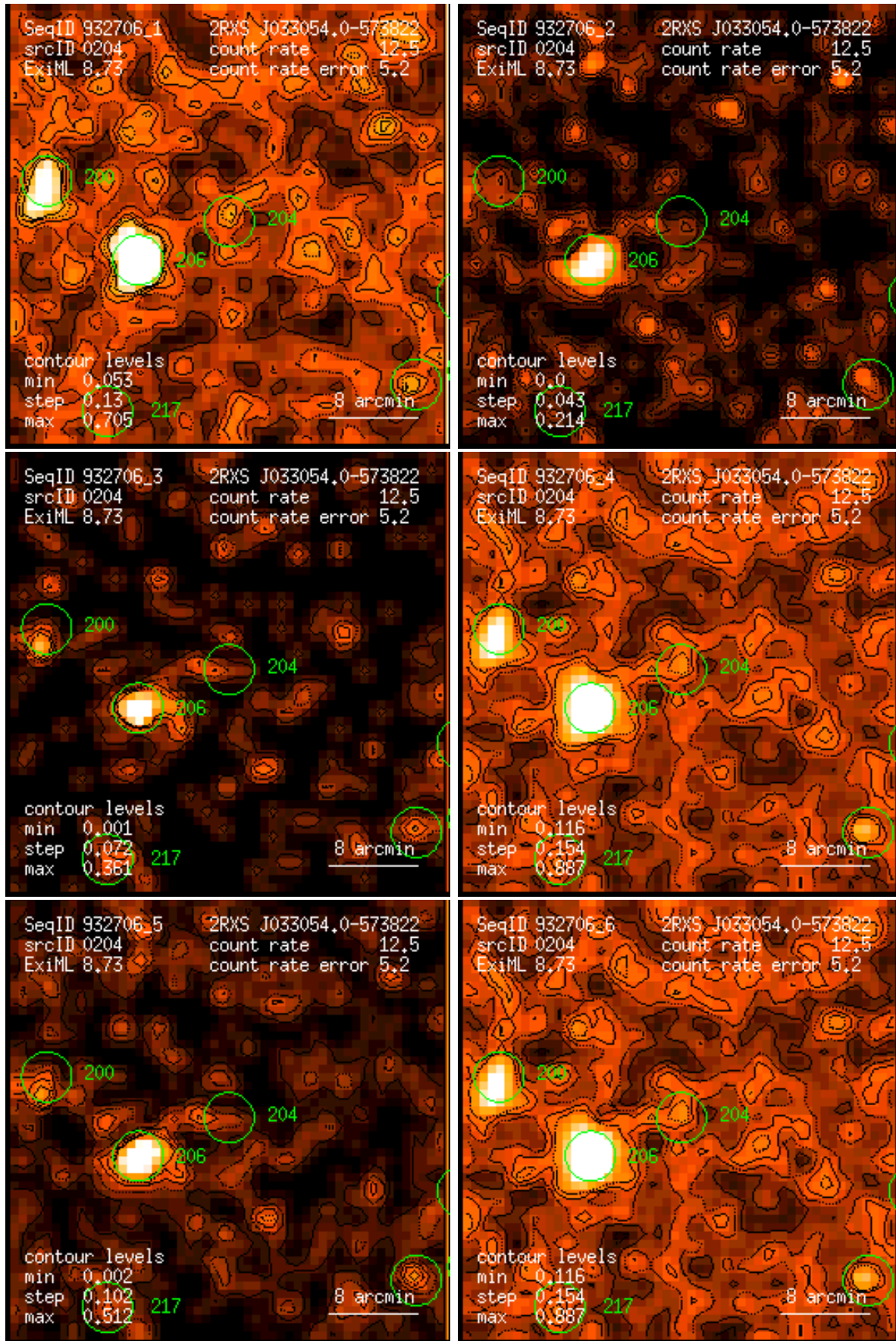
Figure 204: RASS 932706: detection 0204: band rate images, Gaussian filter: (1) PSPC channels 11 – 41, (2) 52 – 90, (3) 91 – 201, (4) 11 – 235, (5) 52 – 201, (6) 11 – 201. Broad band rates in counts/ks. Band rate contour levels in counts/ks/arcmin 2 .
