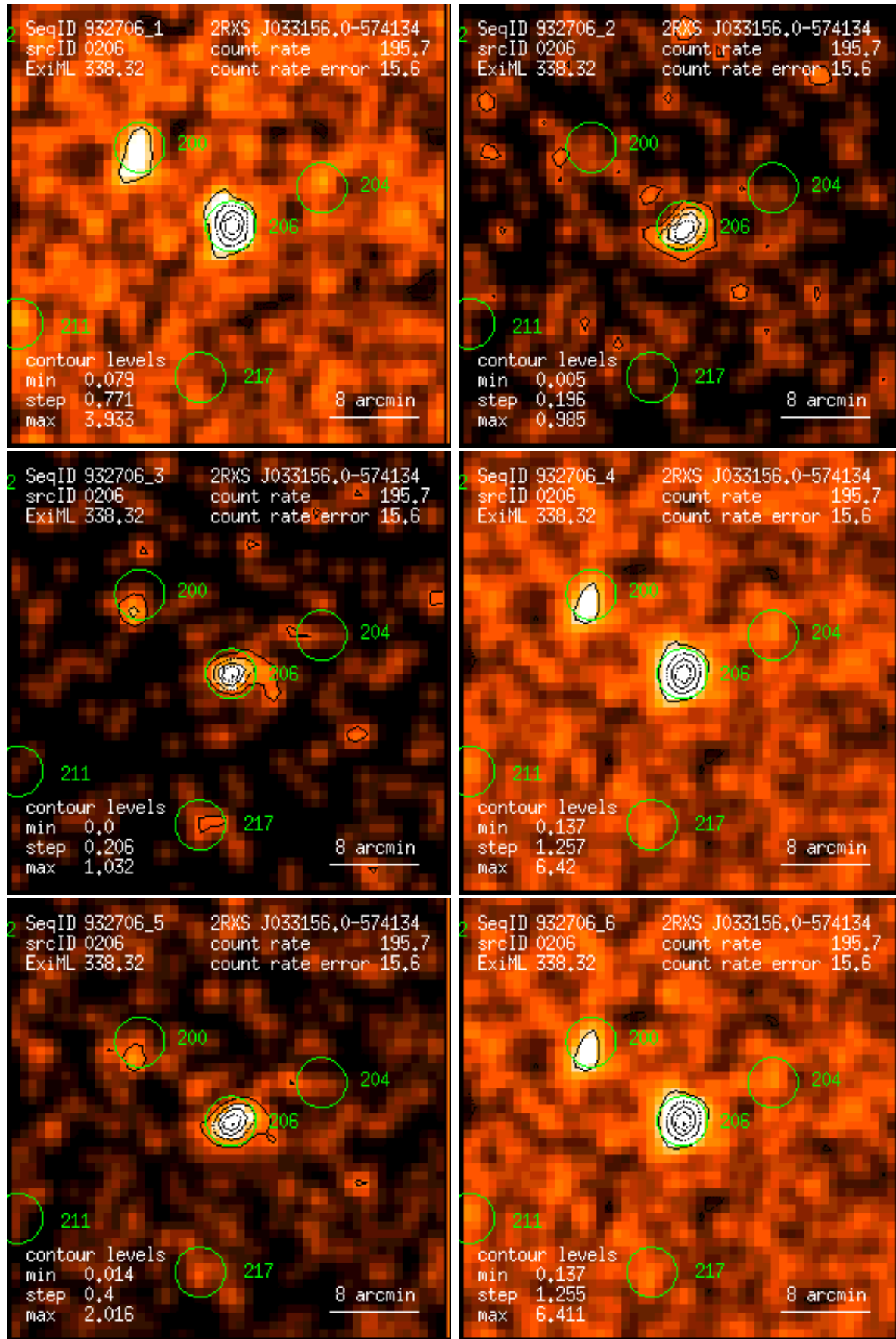
Figure 206: RASS 932706: detection 0206: band rate images, Gaussian filter: (1) PSPC channels 11 – 41, (2) 52 – 90, (3) 91 – 201, (4) 11 – 235, (5) 52 – 201, (6) 11 – 201. Broad band rates in counts/ks. Band rate contour levels in counts/ks/arcmin 2 .
