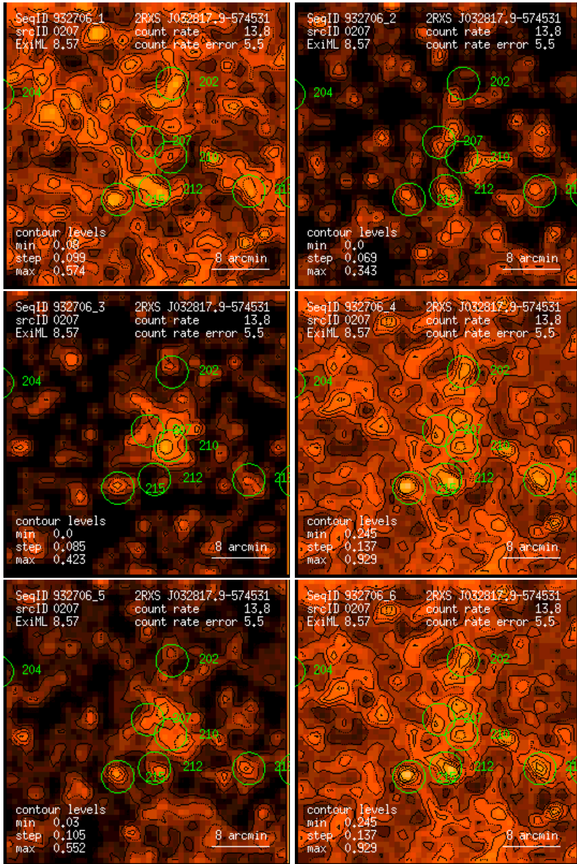
Figure 207: RASS 932706: detection 0207: band rate images, Gaussian filter: (1) PSPC channels 11 – 41, (2) 52 – 90, (3) 91 – 201, (4) 11 – 235, (5) 52 – 201, (6) 11 – 201. Broad band rates in counts/ks. Band rate contour levels in counts/ks/arcmin 2 .
