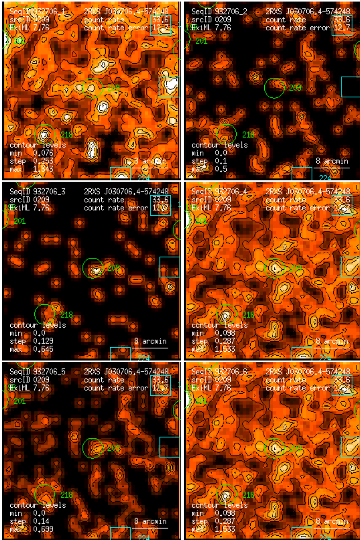
Figure 209: RASS 932706: detection 0209: band rate images, Gaussian filter: (1) PSPC channels 11 – 41, (2) 52 – 90, (3) 91 – 201, (4) 11 – 235, (5) 52 – 201, (6) 11 – 201. Broad band rates in counts/ks. Band rate contour levels in counts/ks/arcmin 2 .
