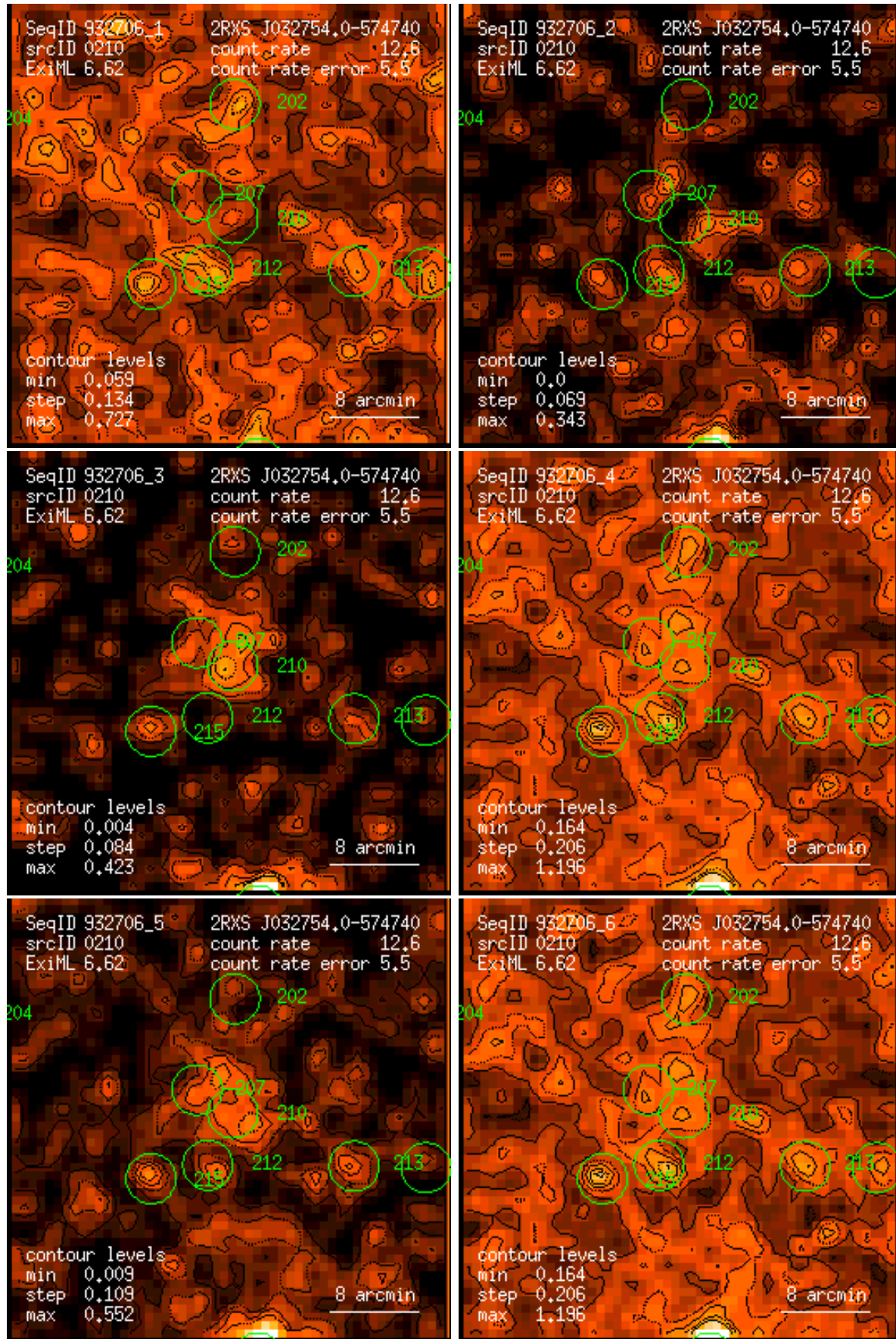
Figure 210: RASS 932706: detection 0210: band rate images, Gaussian filter: (1) PSPC channels 11 – 41, (2) 52 – 90, (3) 91 – 201, (4) 11 – 235, (5) 52 – 201, (6) 11 – 201. Broad band rates in counts/ks. Band rate contour levels in counts/ks/arcmin 2 .
