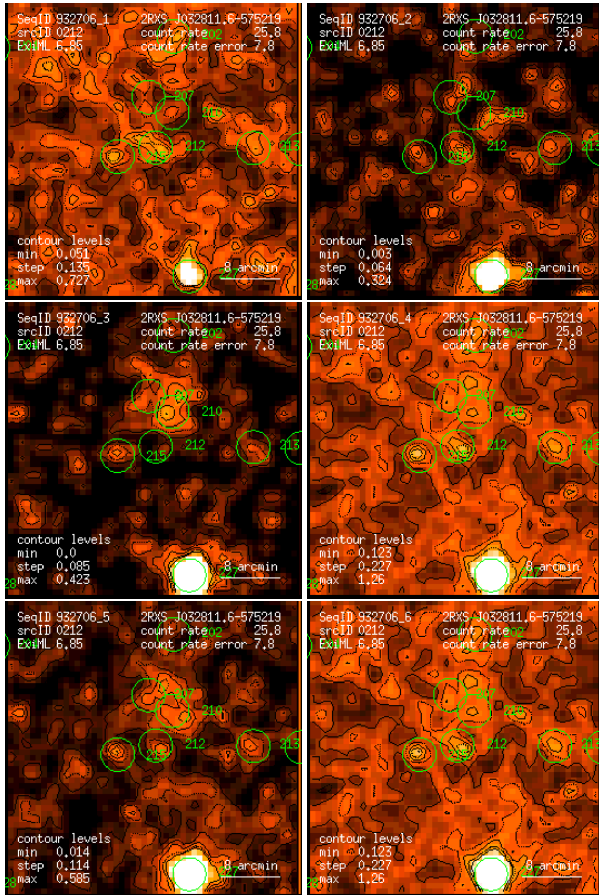
Figure 212: RASS 932706: detection 0212: band rate images, Gaussian filter: (1) PSPC channels 11 – 41, (2) 52 – 90, (3) 91 – 201, (4) 11 – 235, (5) 52 – 201, (6) 11 – 201. Broad band rates in counts/ks. Band rate contour levels in counts/ks/arcmin 2 .
