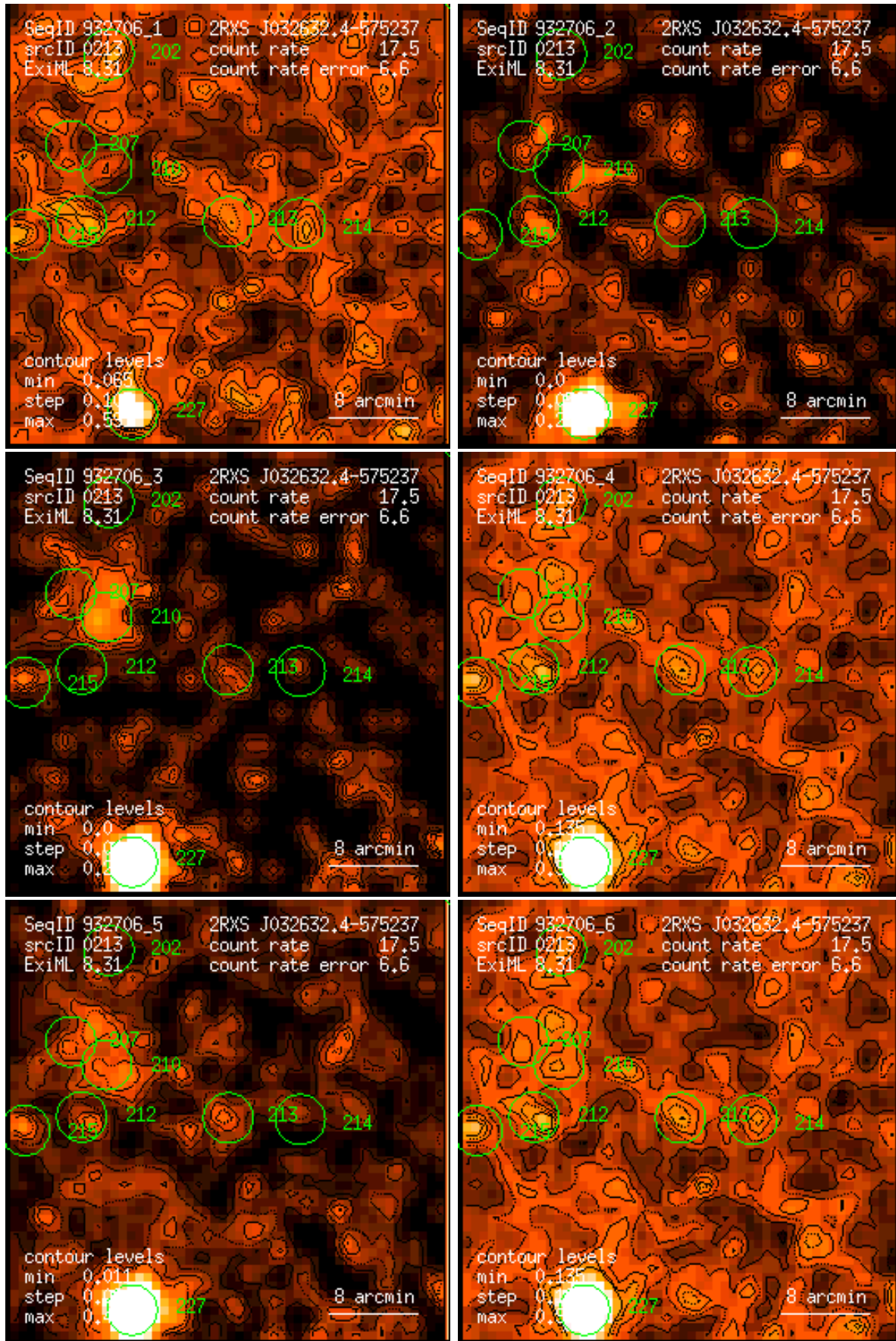
Figure 213: RASS 932706: detection 0213: band rate images, Gaussian filter: (1) PSPC channels 11 – 41, (2) 52 – 90, (3) 91 – 201, (4) 11 – 235, (5) 52 – 201, (6) 11 – 201. Broad band rates in counts/ks. Band rate contour levels in counts/ks/arcmin 2 .
