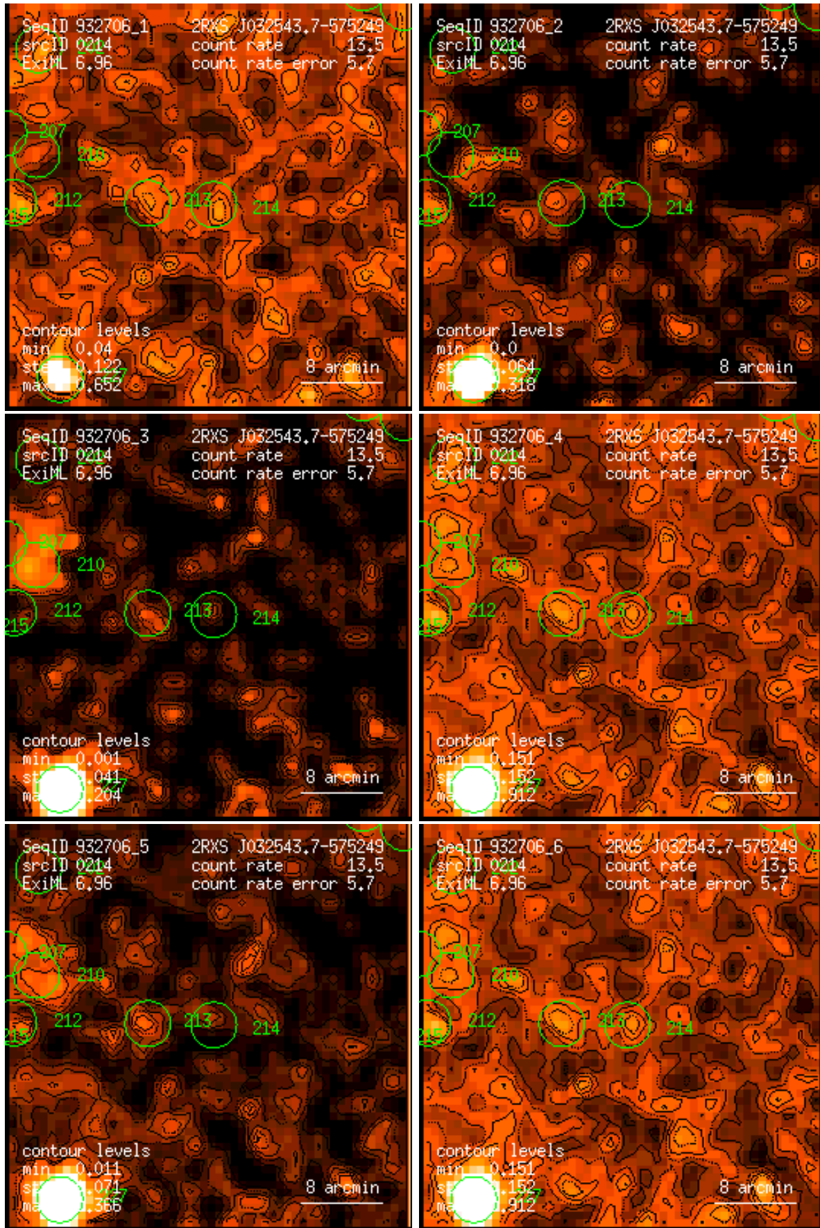
Figure 214: RASS 932706: detection 0214: band rate images, Gaussian filter: (1) PSPC channels 11 – 41, (2) 52 – 90, (3) 91 – 201, (4) 11 – 235, (5) 52 – 201, (6) 11 – 201. Broad band rates in counts/ks. Band rate contour levels in counts/ks/arcmin 2 .
