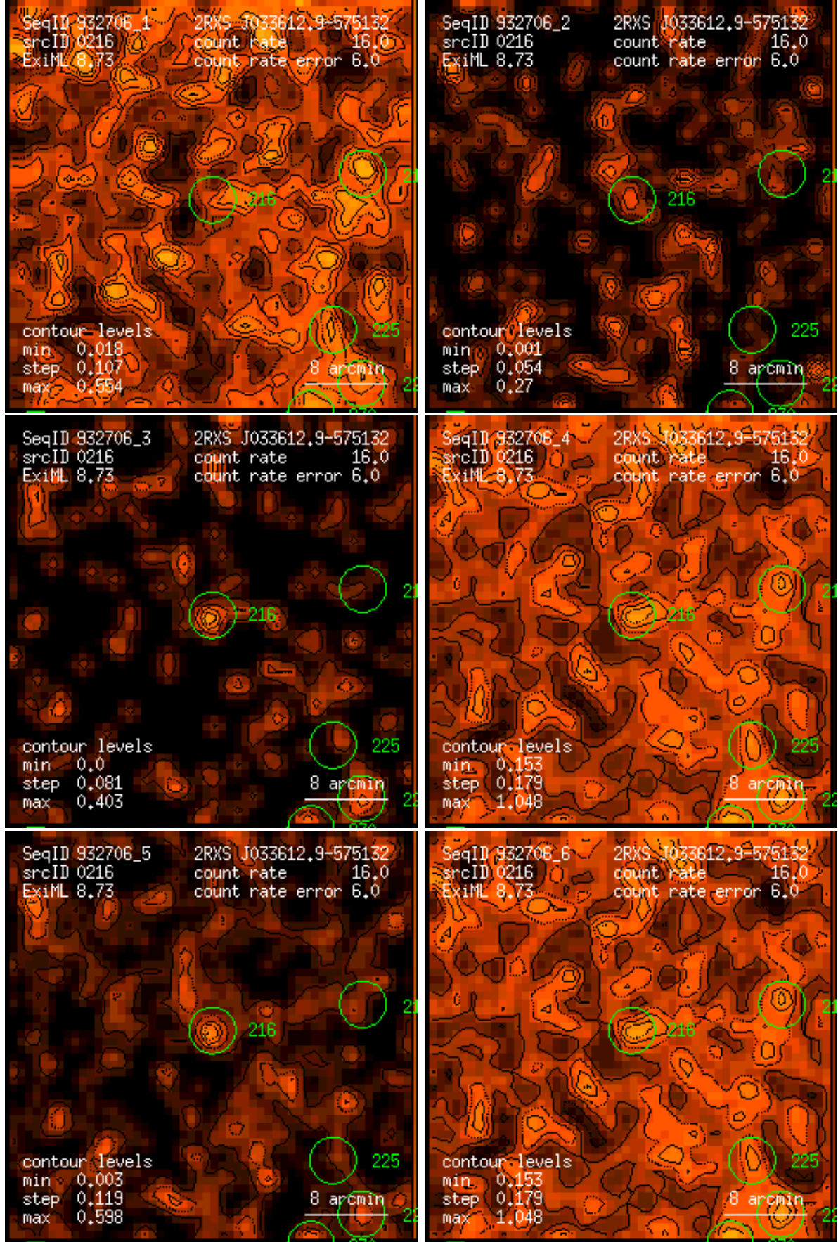
Figure 216: RASS 932706: detection 0216: band rate images, Gaussian filter: (1) PSPC channels 11 – 41, (2) 52 – 90, (3) 91 – 201, (4) 11 – 235, (5) 52 – 201, (6) 11 – 201. Broad band rates in counts/ks. Band rate contour levels in counts/ks/arcmin 2 .
